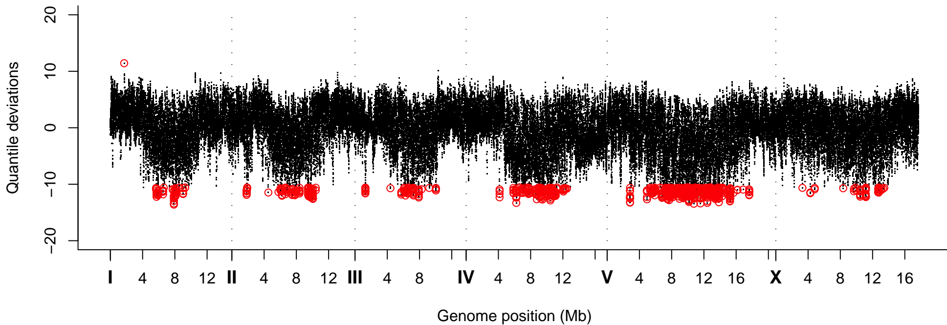
Quantile Deviations, Strain VC20203
