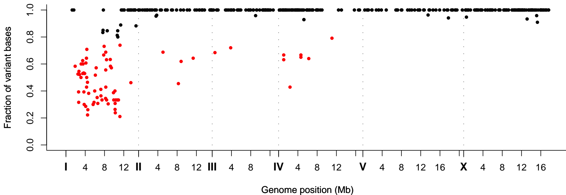
Fraction of Variant Bases at Position, Strain VC20203
