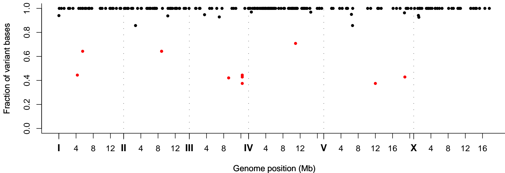
Fraction of Variant Bases at Position, Strain VC20205
