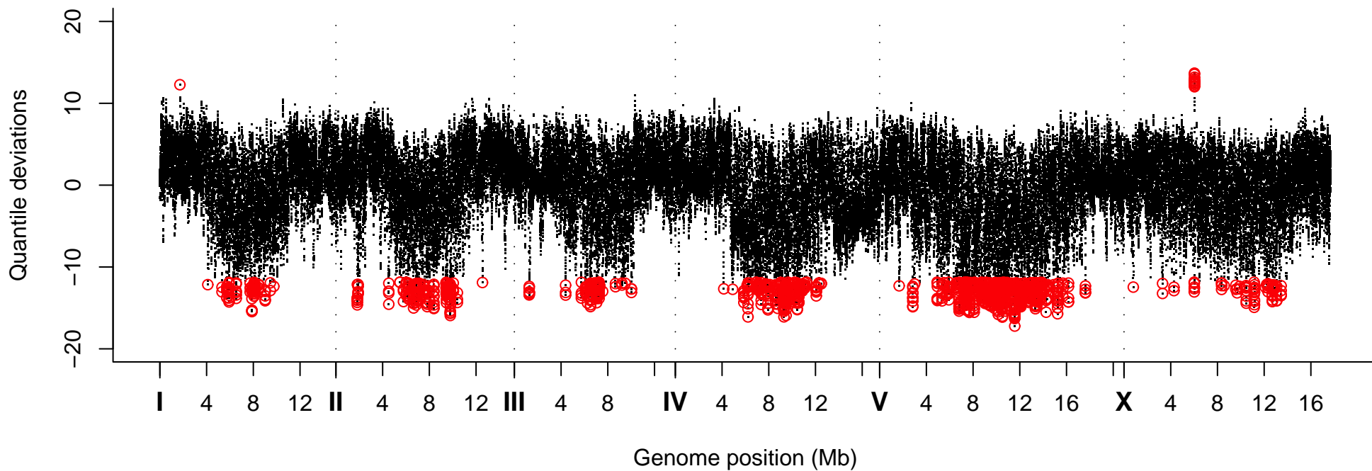
Quantile Deviations, Strain VC20205
