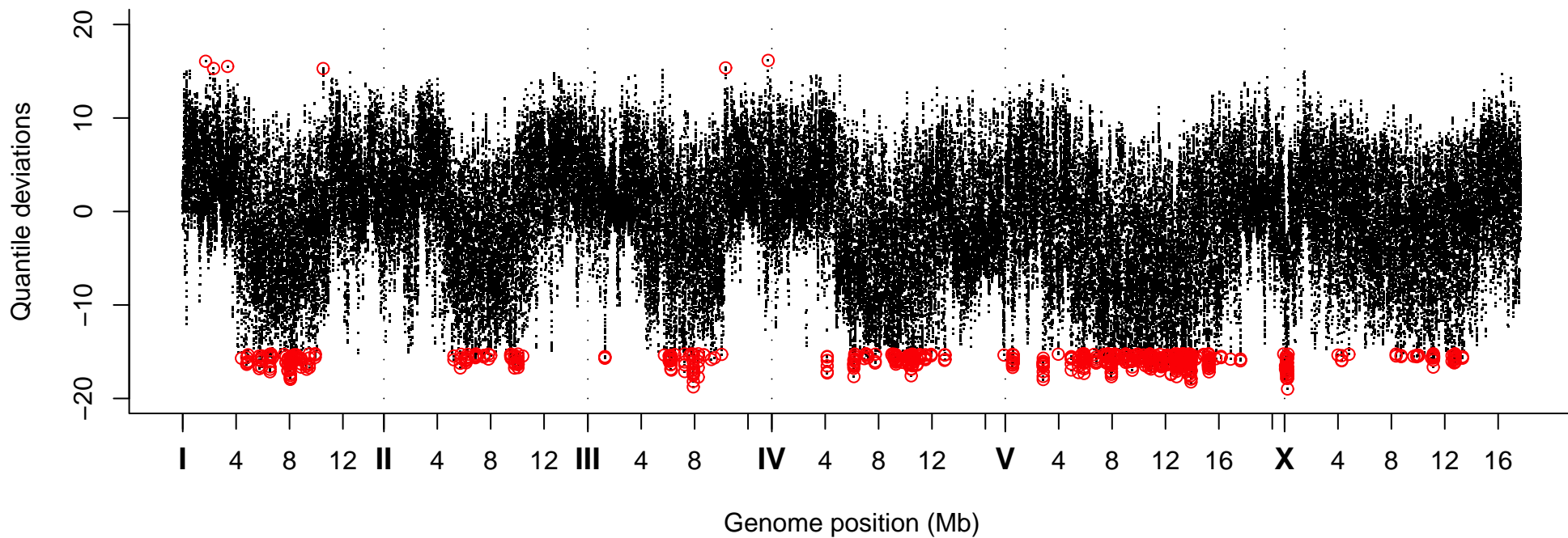
Quantile Deviations, Strain VC20206
