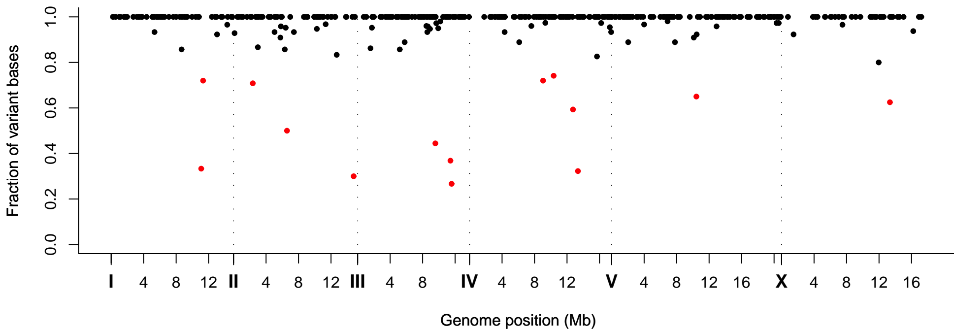
Fraction of Variant Bases at Position, Strain VC20206
