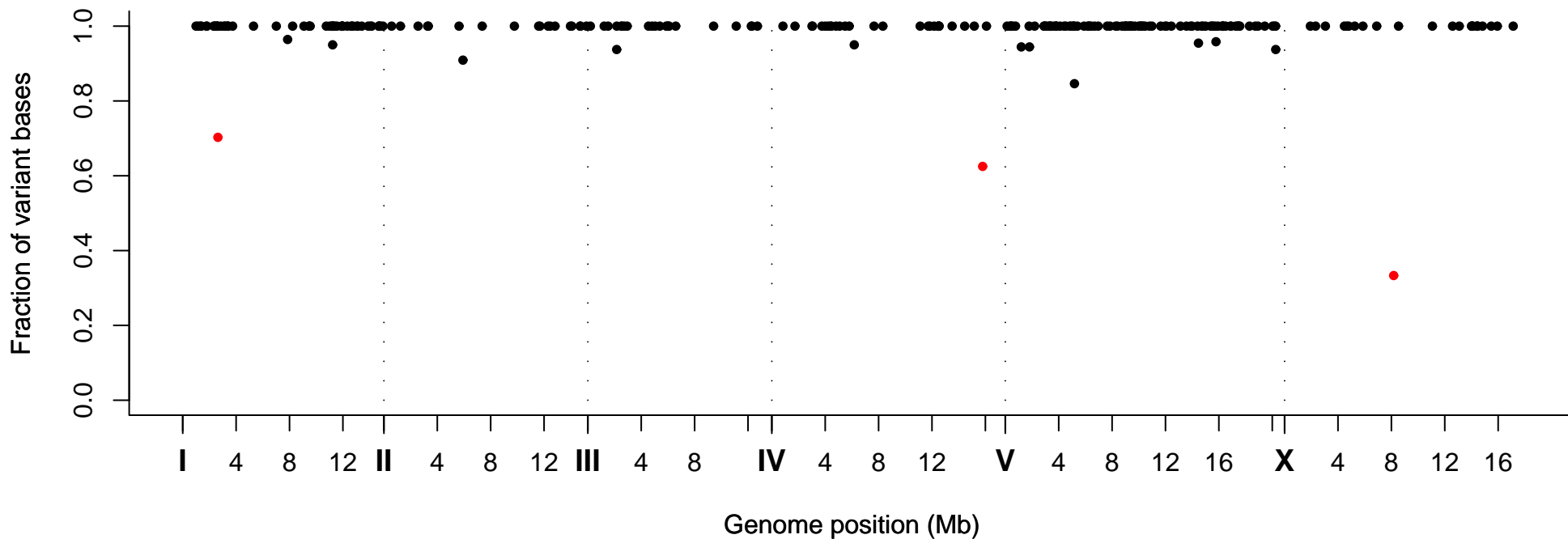
Fraction of Variant Bases at Position, Strain VC20211
