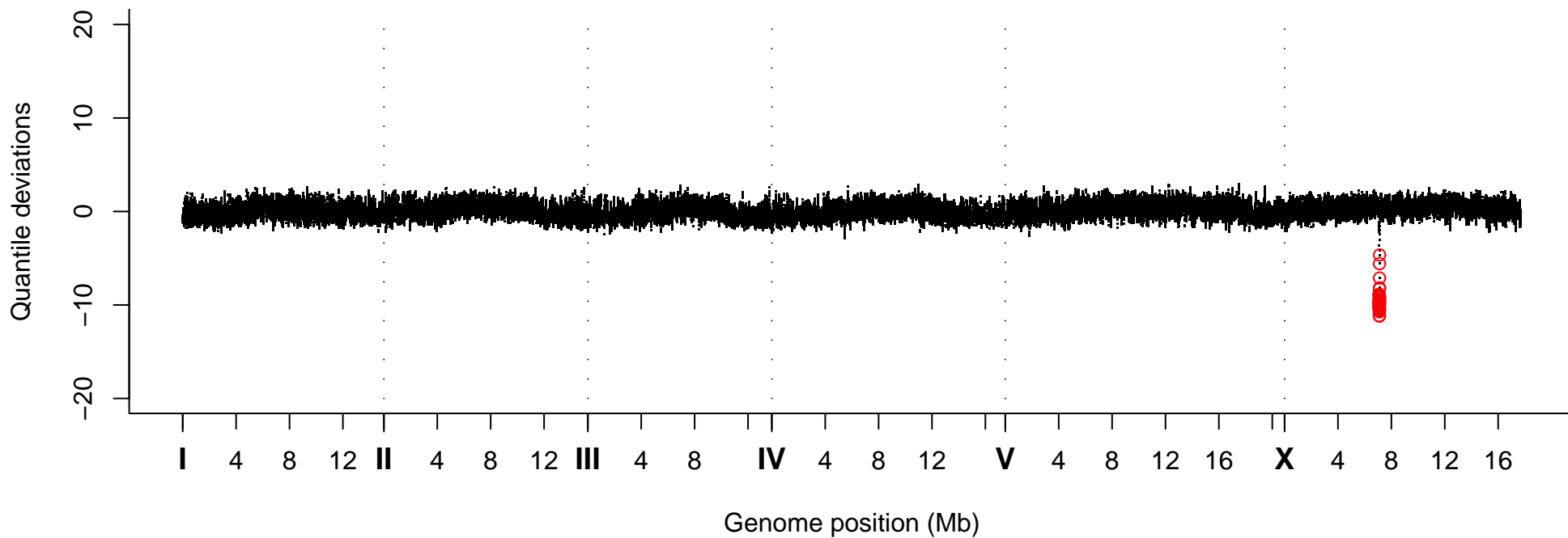
Quantile Deviations, Strain VC20211
