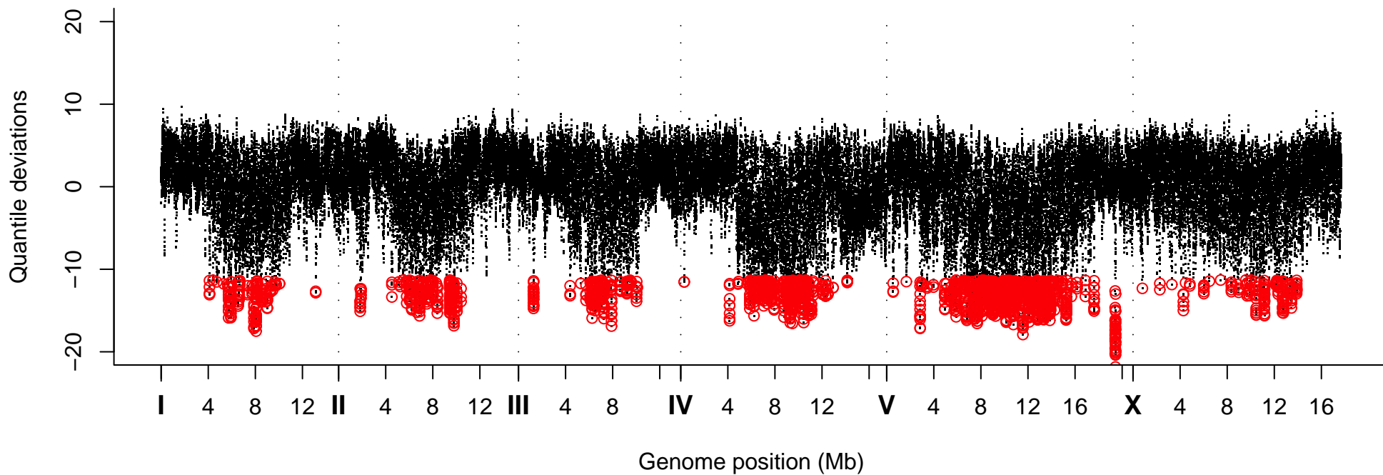
Quantile Deviations, Strain VC20212
