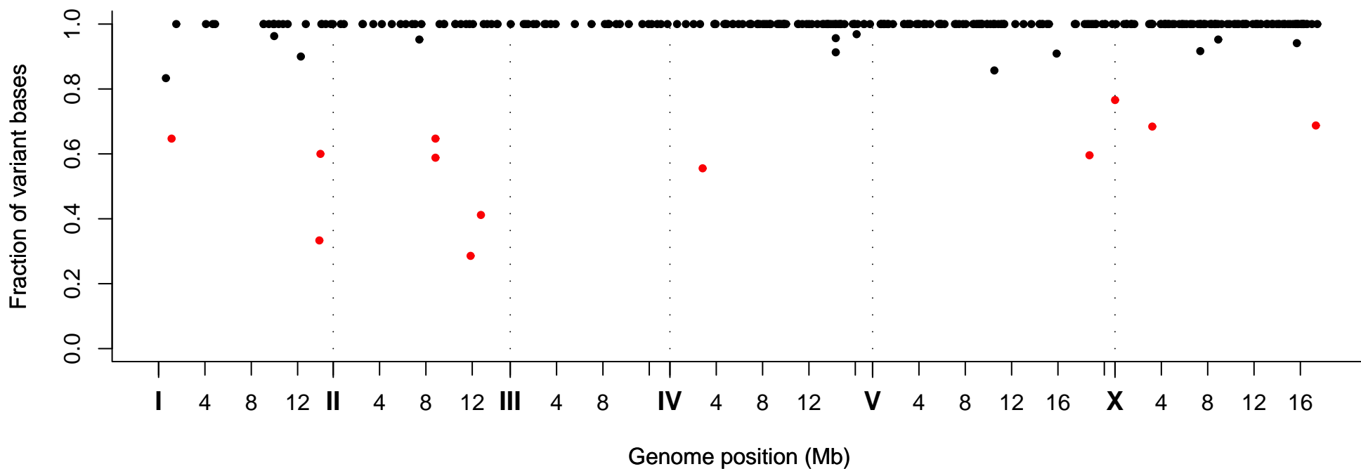
Fraction of Variant Bases at Position, Strain VC20212
