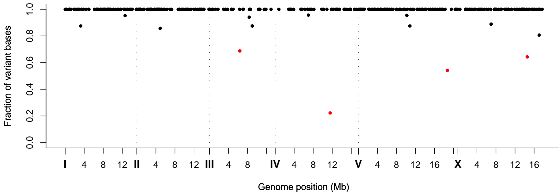
Fraction of Variant Bases at Position, Strain VC20213
