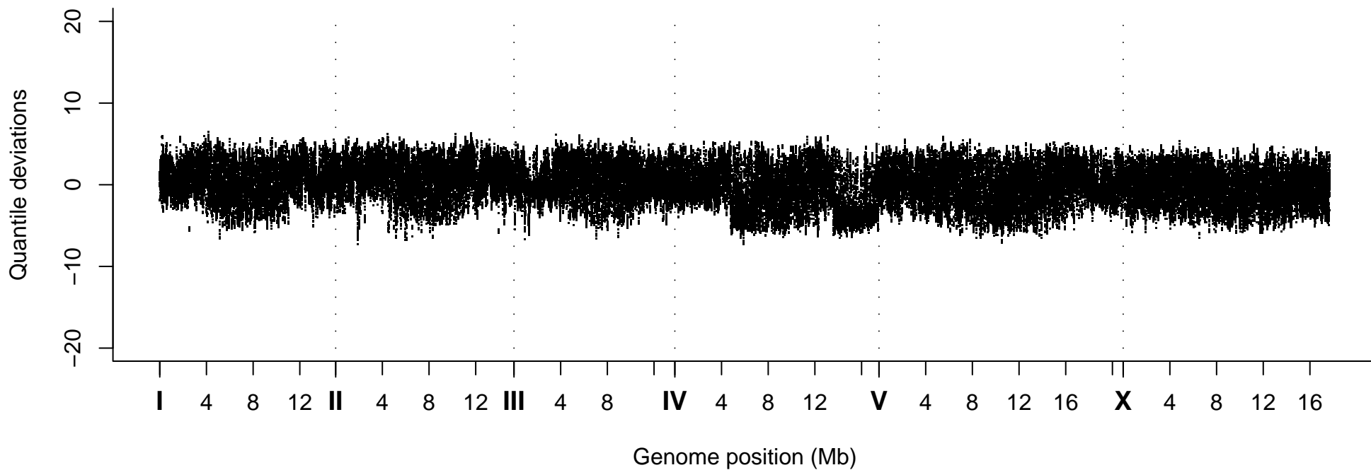
Quantile Deviations, Strain VC20213
