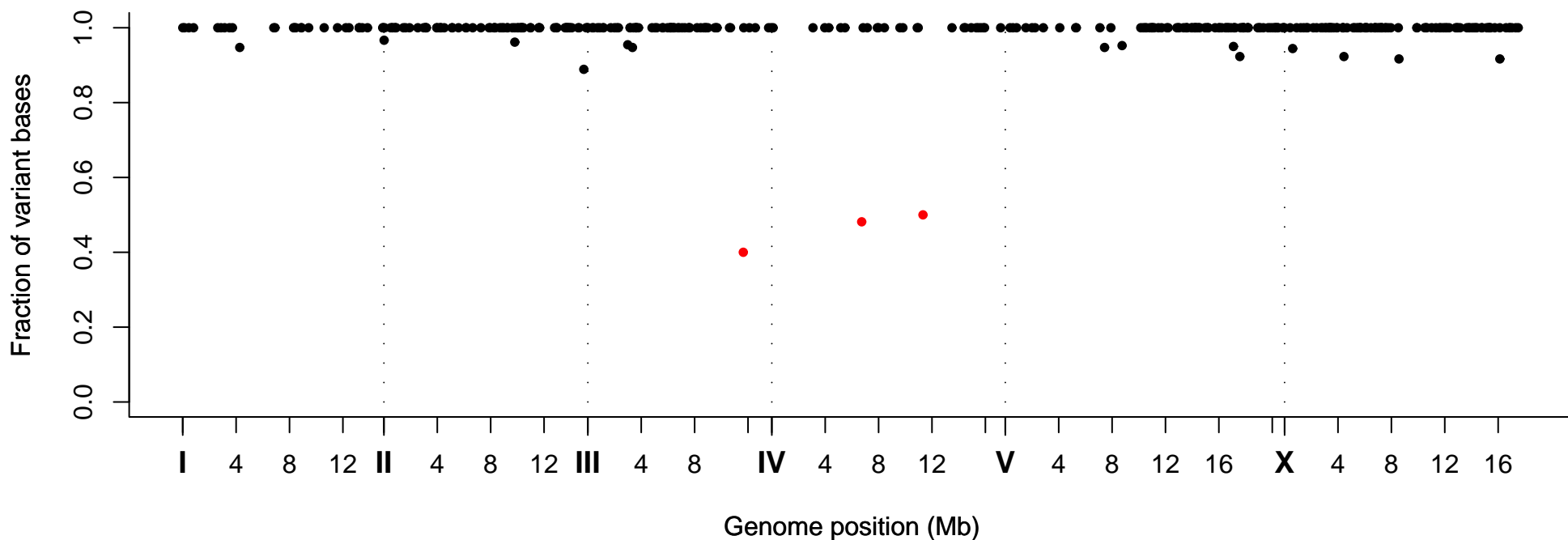
Fraction of Variant Bases at Position, Strain VC20218
