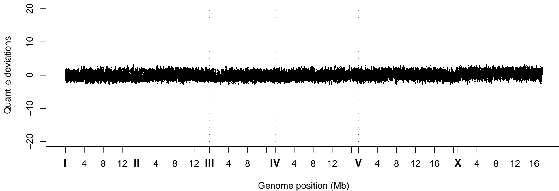
Quantile Deviations, Strain VC20218
