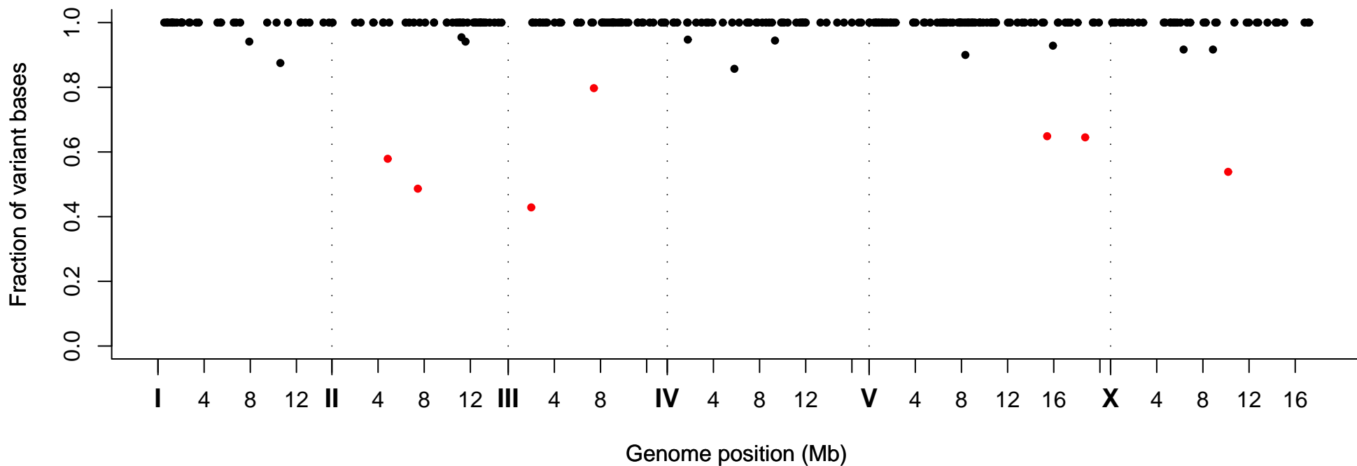
Fraction of Variant Bases at Position, Strain VC20221
