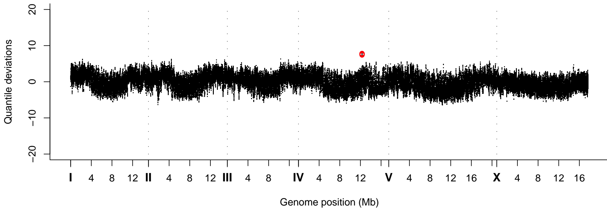
Quantile Deviations, Strain VC20221
