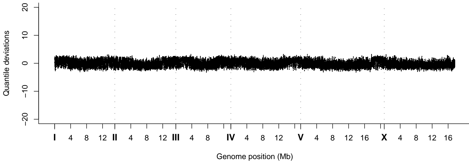
Quantile Deviations, Strain VC20223
