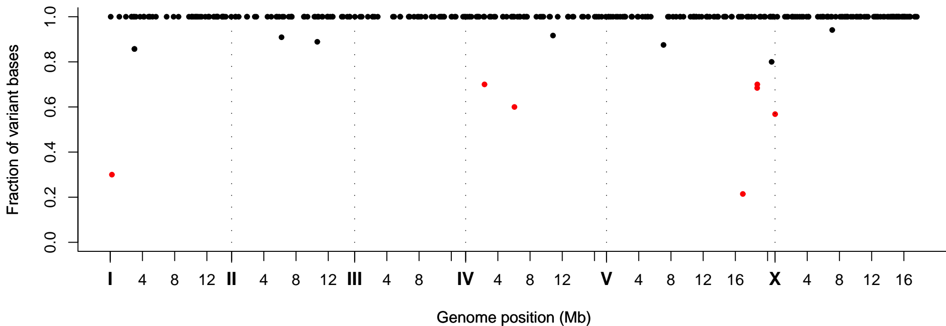
Fraction of Variant Bases at Position, Strain VC20223
