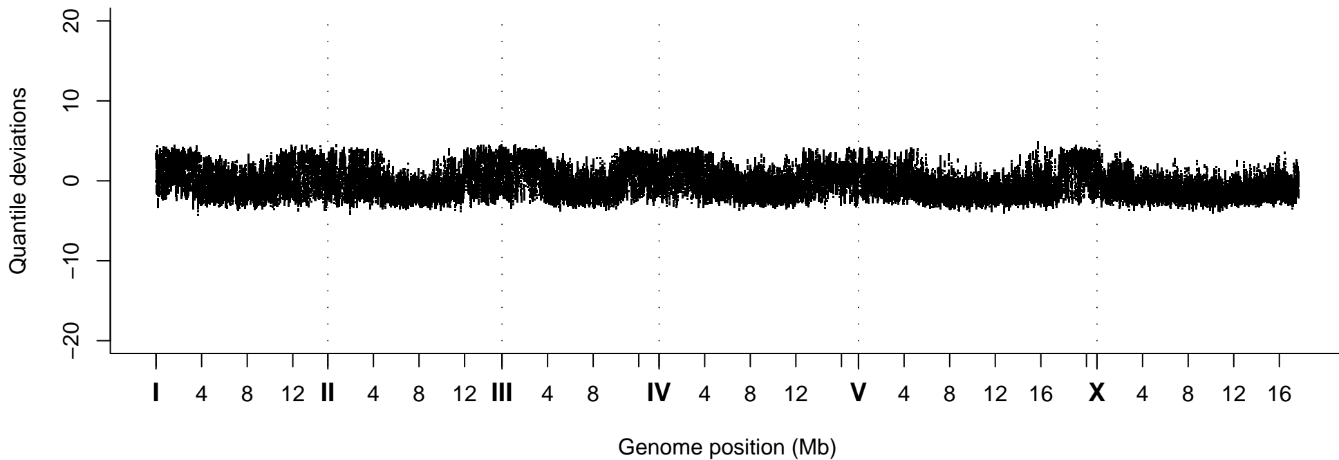
Quantile Deviations, Strain VC20227
