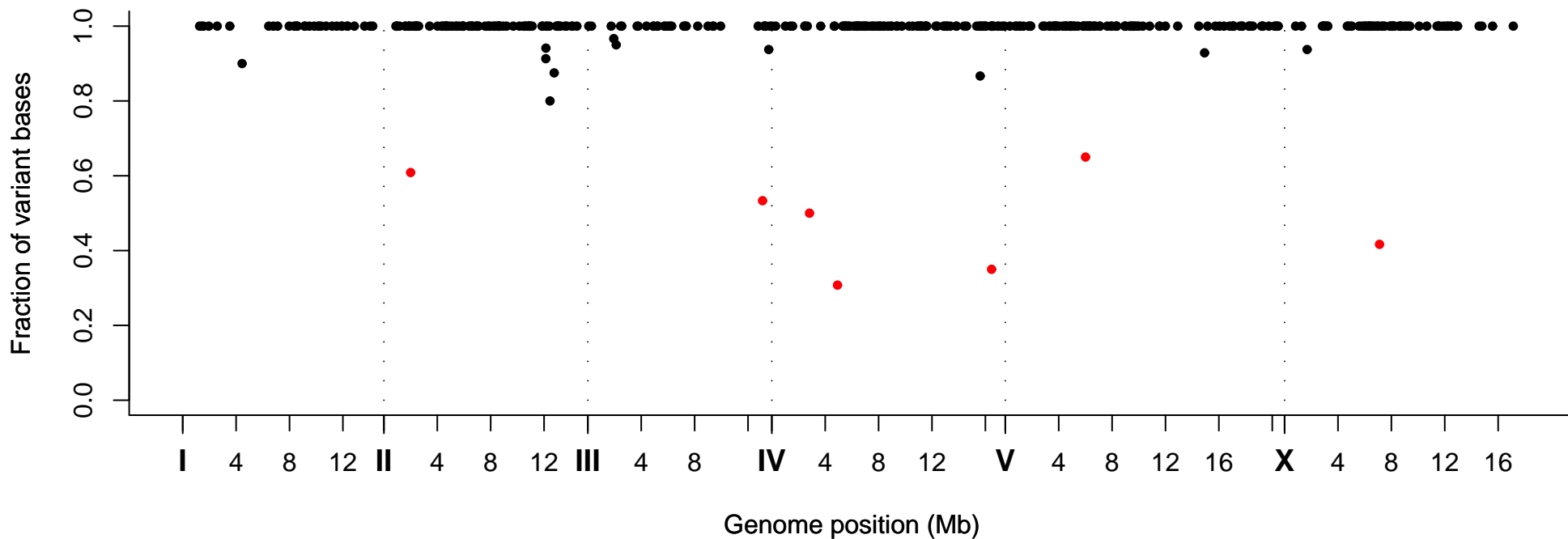
Fraction of Variant Bases at Position, Strain VC20227
