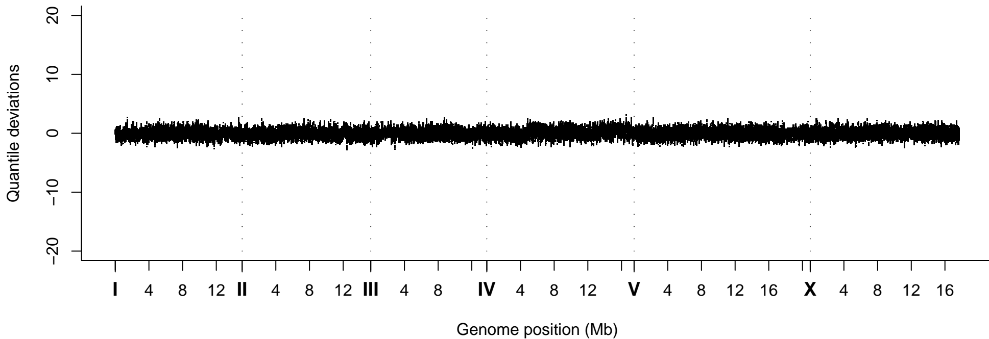
Quantile Deviations, Strain VC20229
