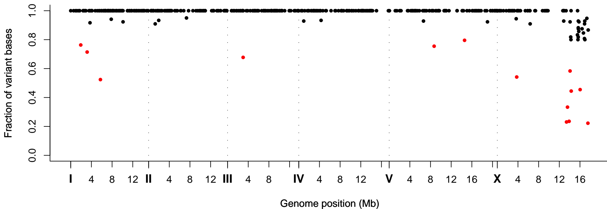
Fraction of Variant Bases at Position, Strain VC20229
