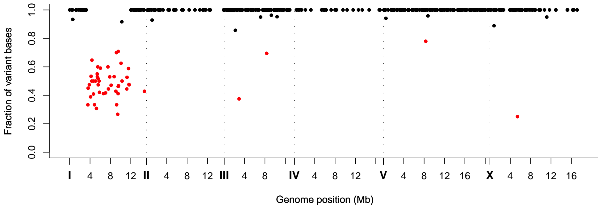
Fraction of Variant Bases at Position, Strain VC20231
