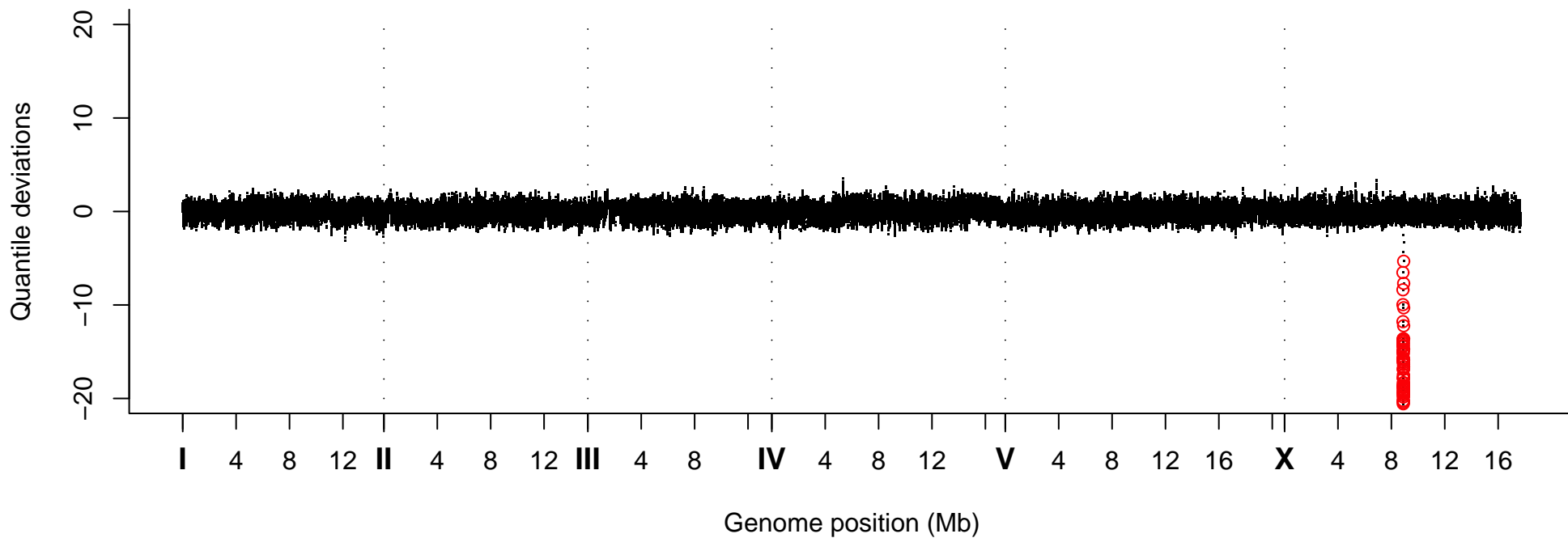
Quantile Deviations, Strain VC20233
