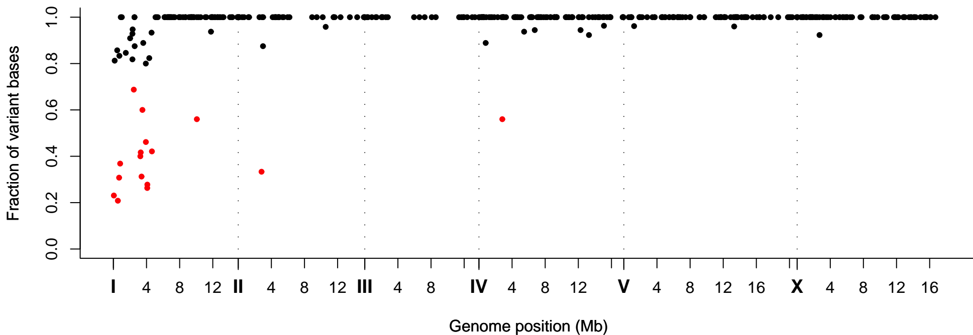
Fraction of Variant Bases at Position, Strain VC20233
