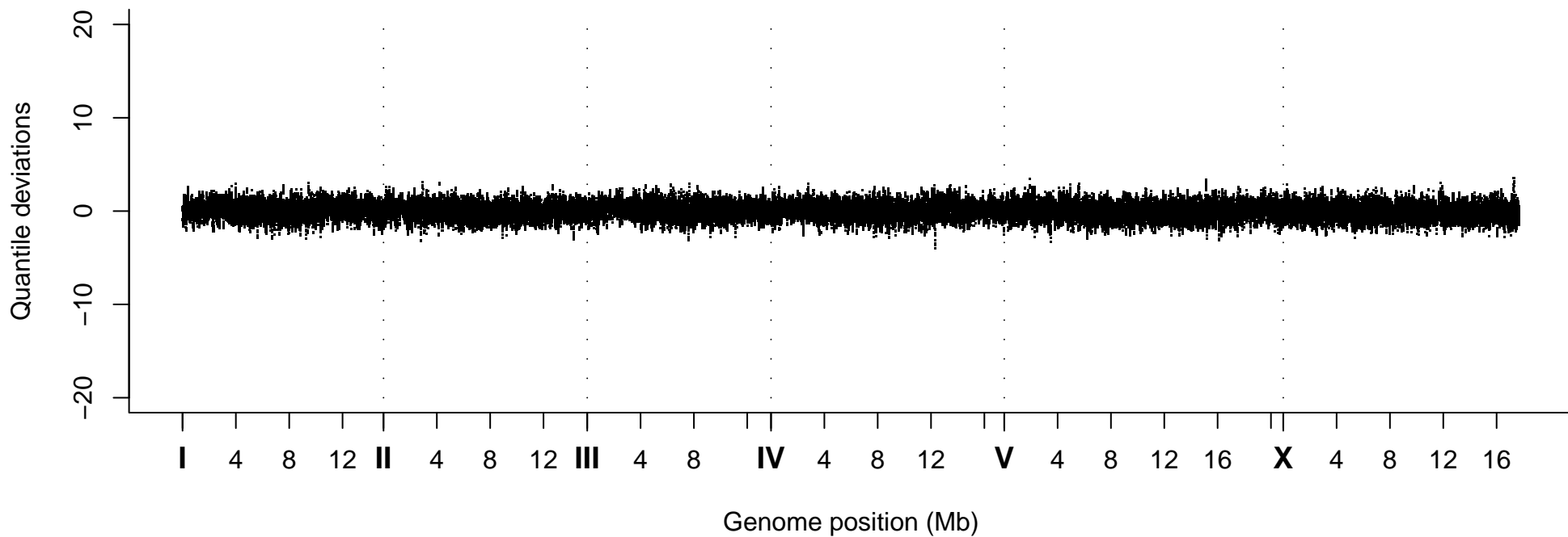
Quantile Deviations, Strain VC20237
