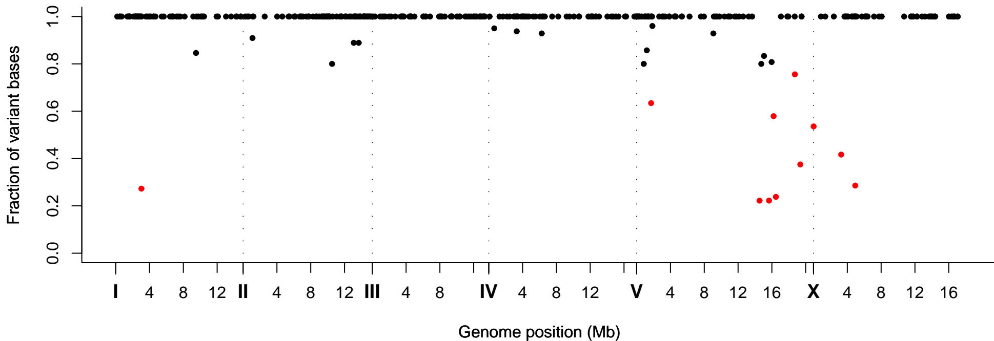
Fraction of Variant Bases at Position, Strain VC20237
