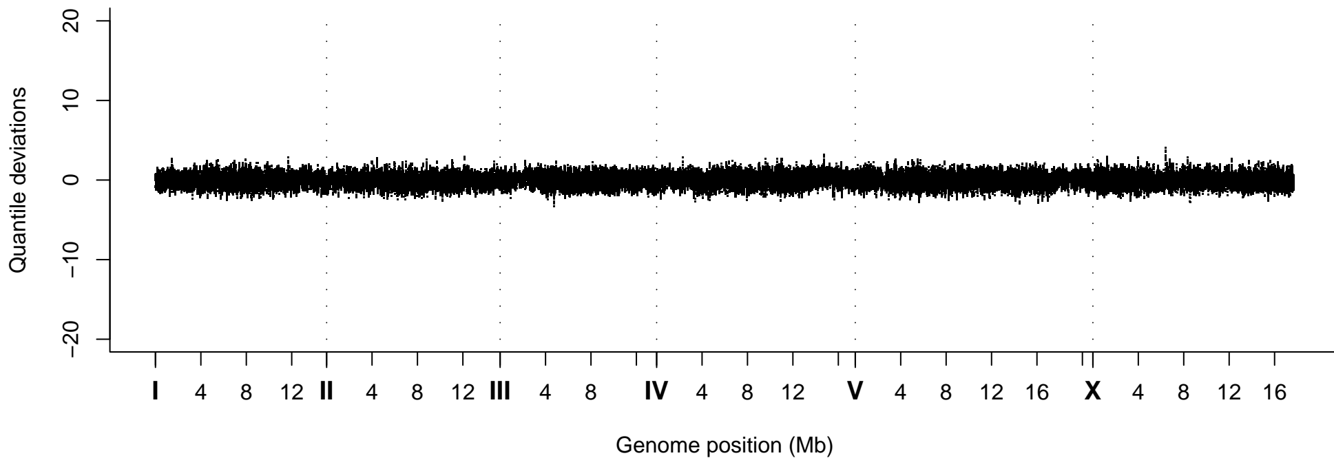
Quantile Deviations, Strain VC20239
