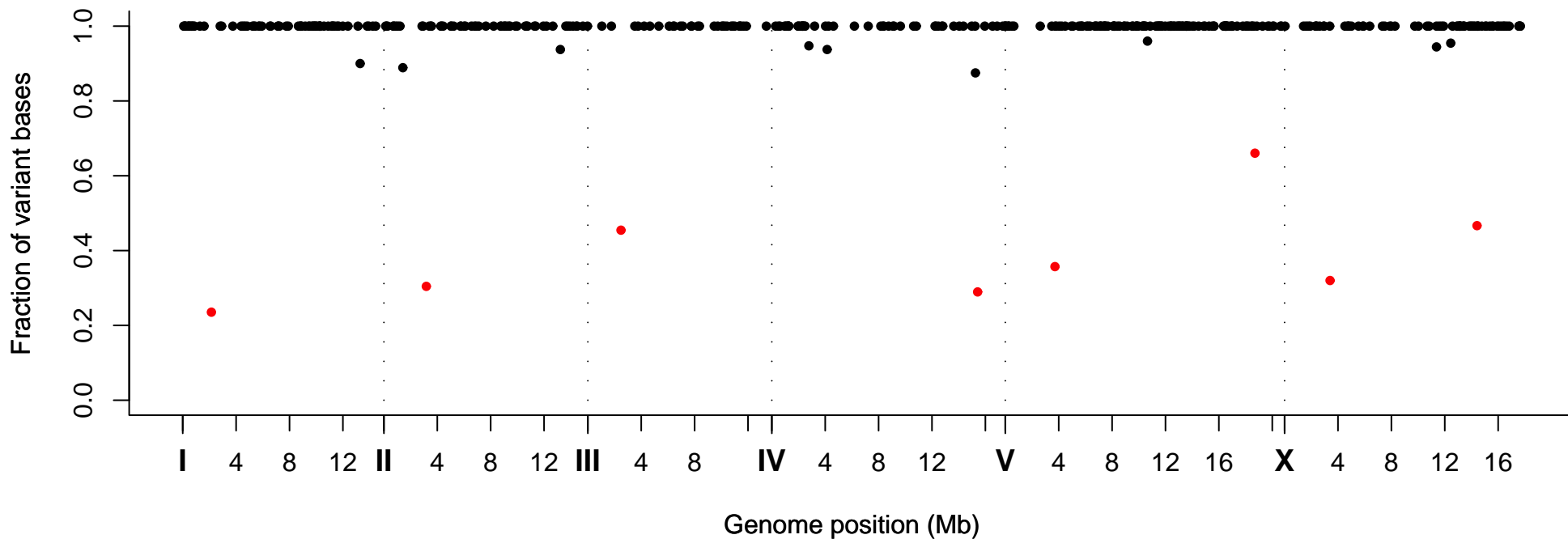
Fraction of Variant Bases at Position, Strain VC20239
