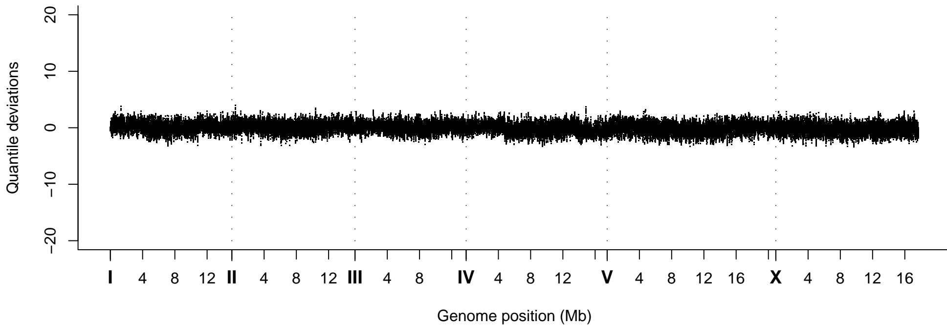
Quantile Deviations, Strain VC20240
