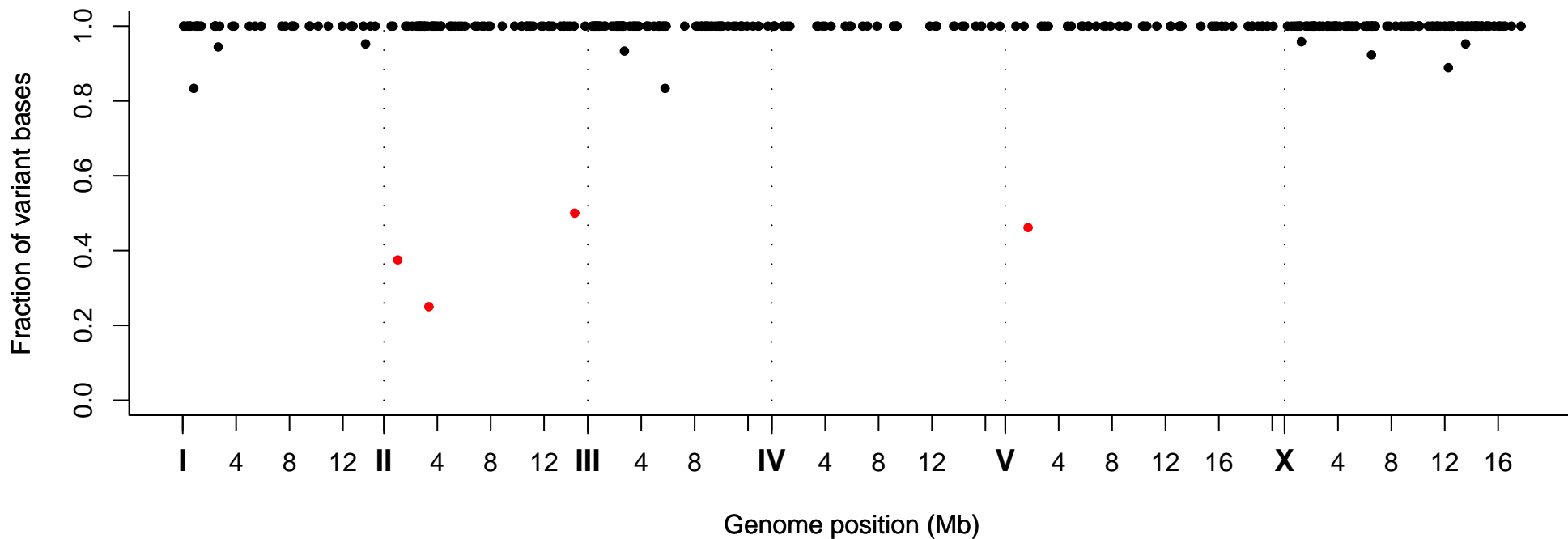
Fraction of Variant Bases at Position, Strain VC20240
