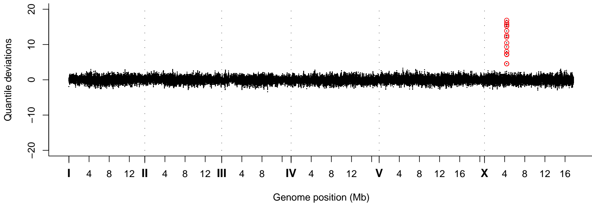
Quantile Deviations, Strain VC20245
