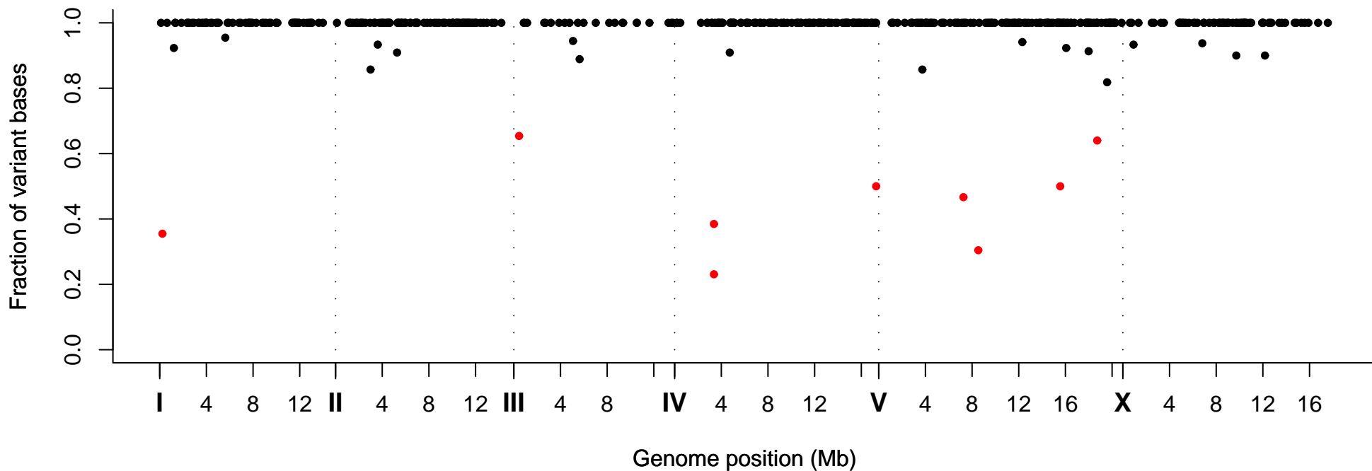
Fraction of Variant Bases at Position, Strain VC20245
