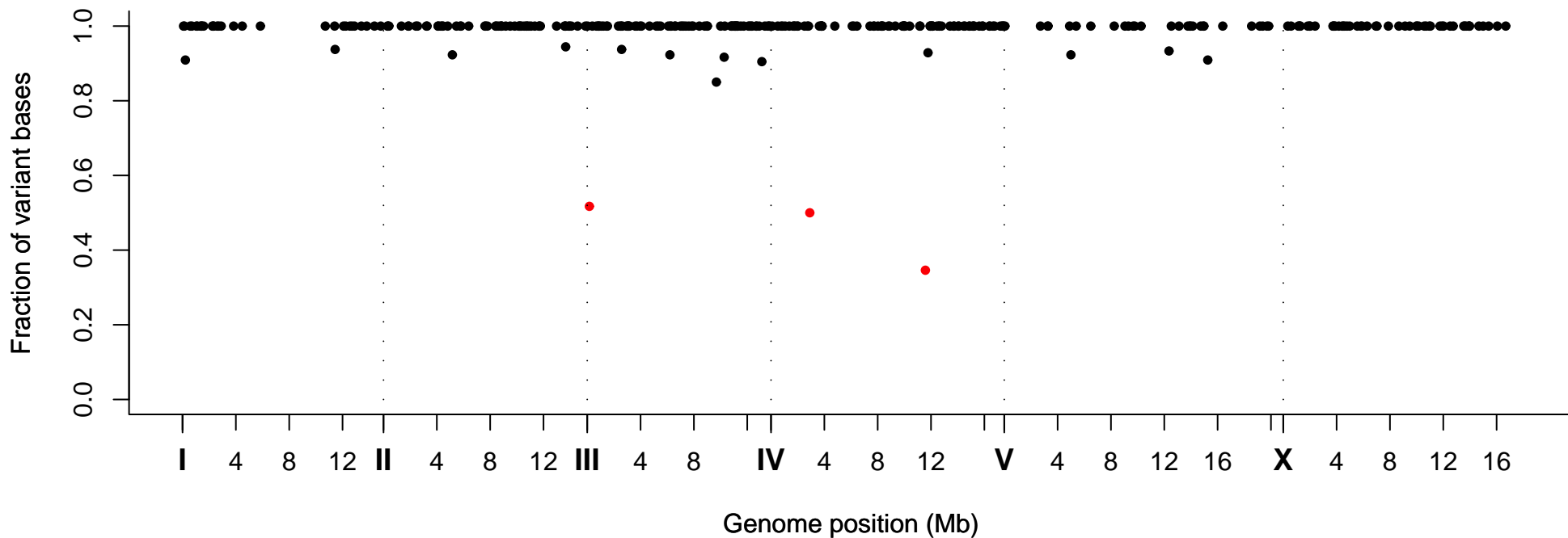
Fraction of Variant Bases at Position, Strain VC20249
