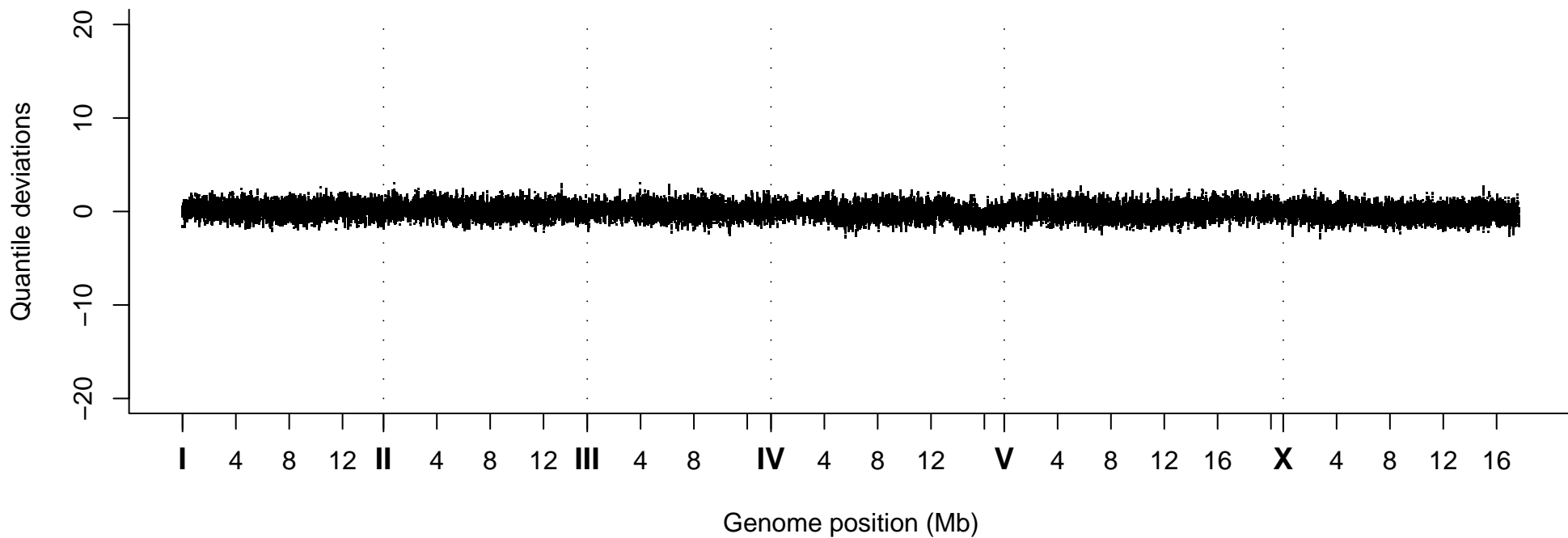
Quantile Deviations, Strain VC20249
