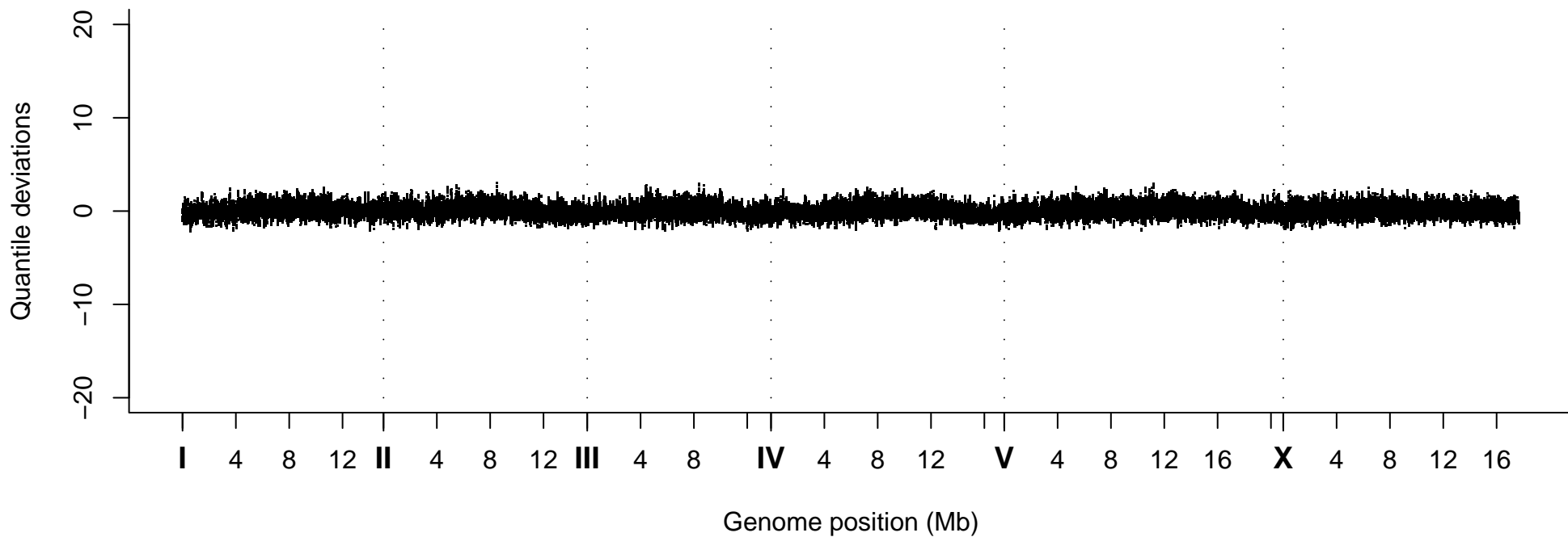
Quantile Deviations, Strain VC20253
