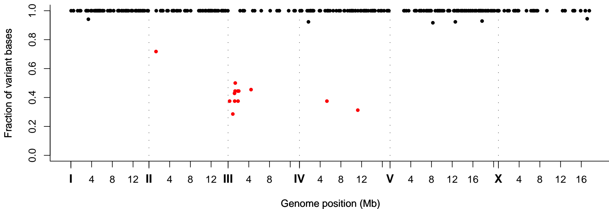
Fraction of Variant Bases at Position, Strain VC20253
