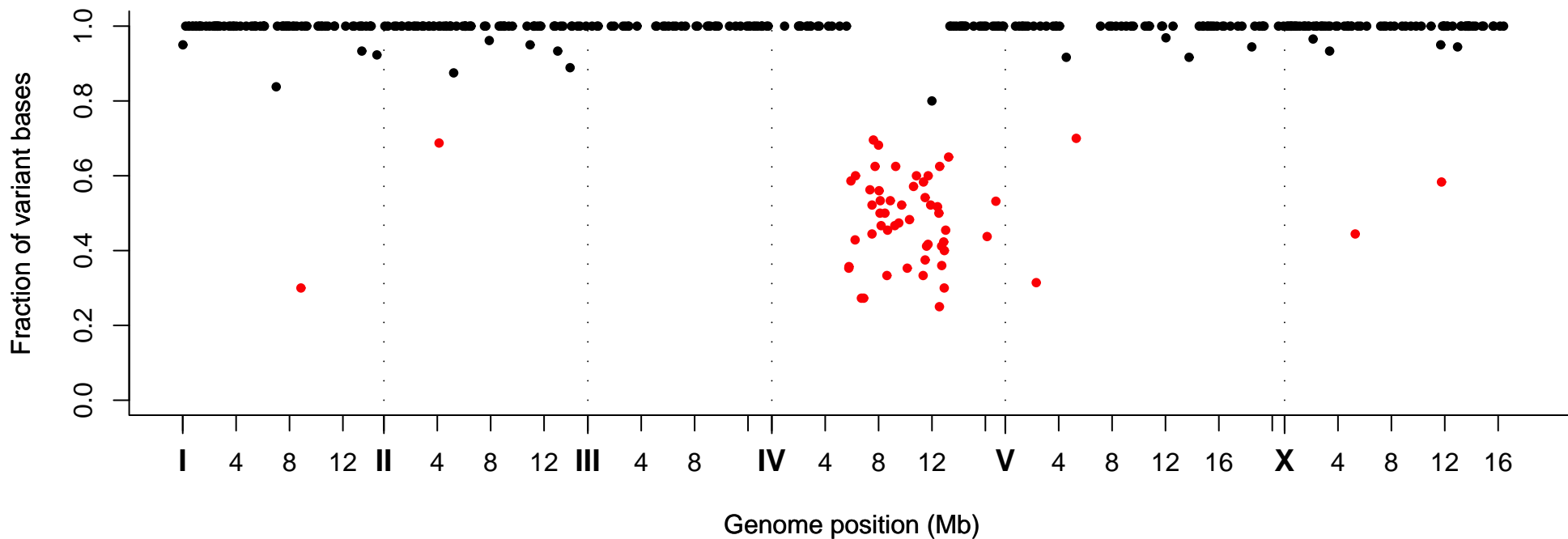
Fraction of Variant Bases at Position, Strain VC20265
