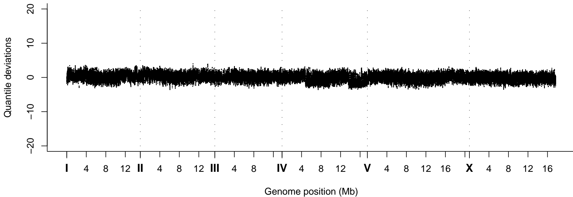
Quantile Deviations, Strain VC20265
