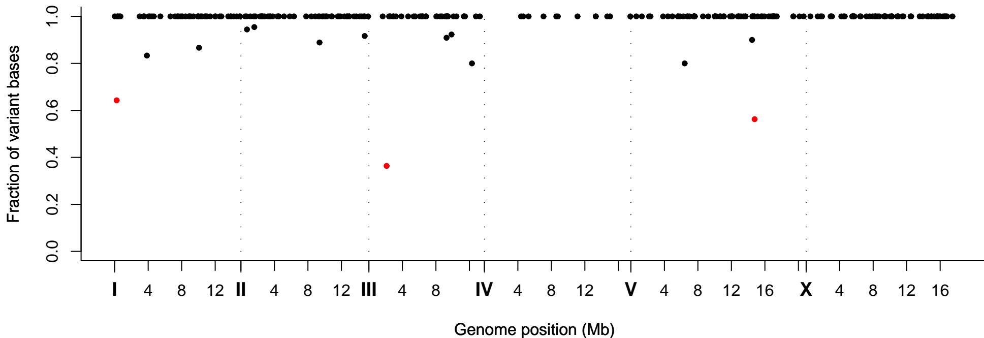
Fraction of Variant Bases at Position, Strain VC20267
