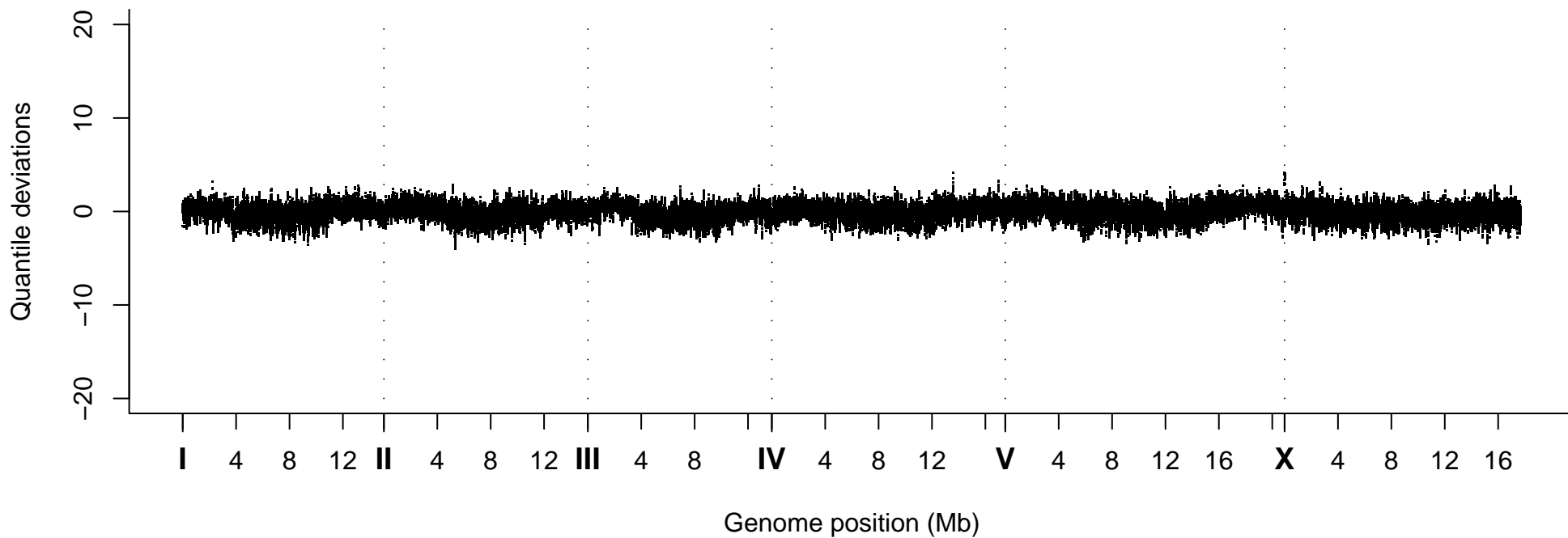
Quantile Deviations, Strain VC20267
