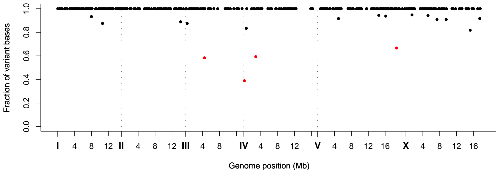
Fraction of Variant Bases at Position, Strain VC20270
