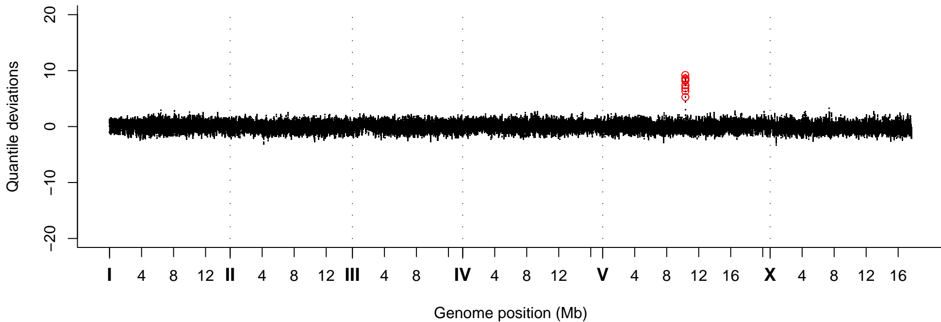
Quantile Deviations, Strain VC20270
