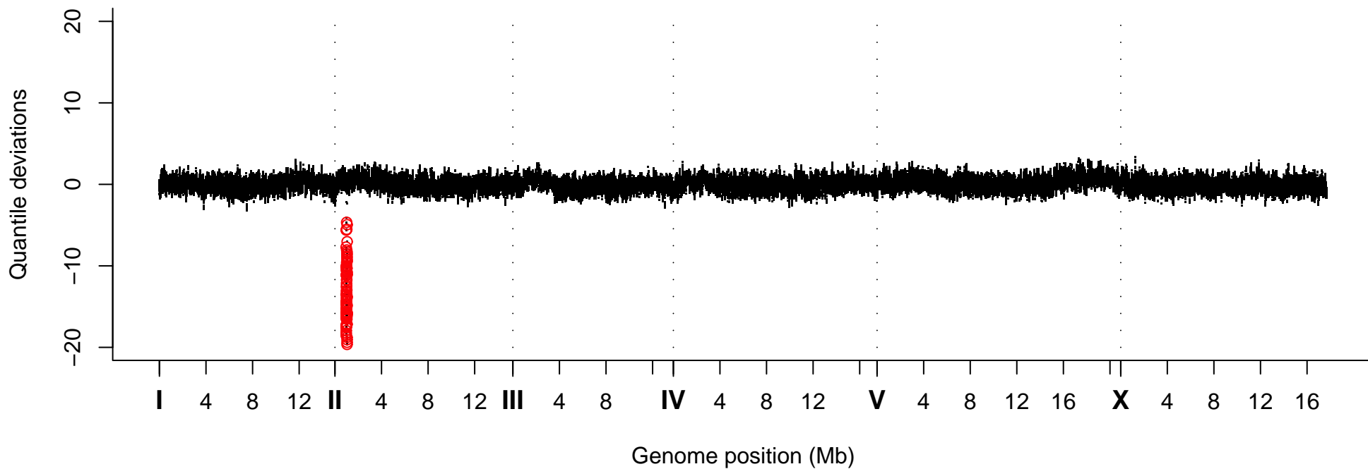
Quantile Deviations, Strain VC20272
