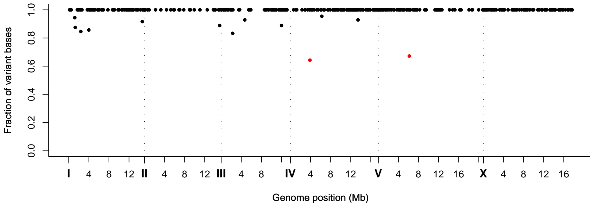
Fraction of Variant Bases at Position, Strain VC20272
