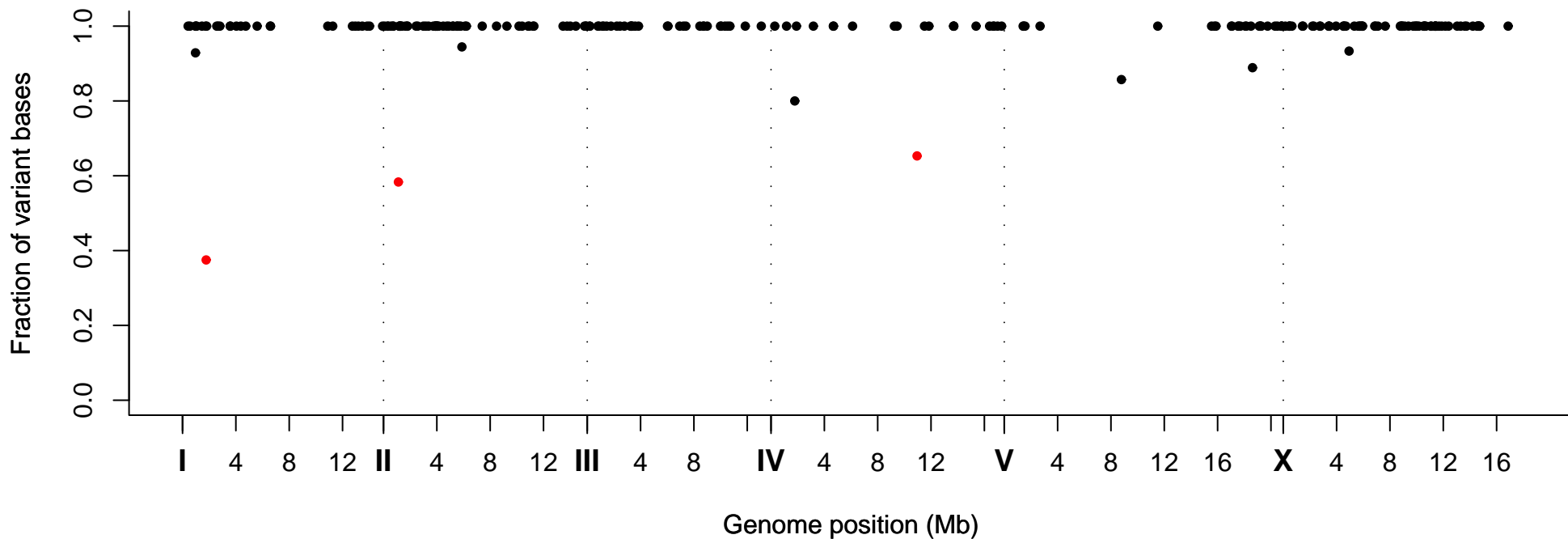
Fraction of Variant Bases at Position, Strain VC20278
