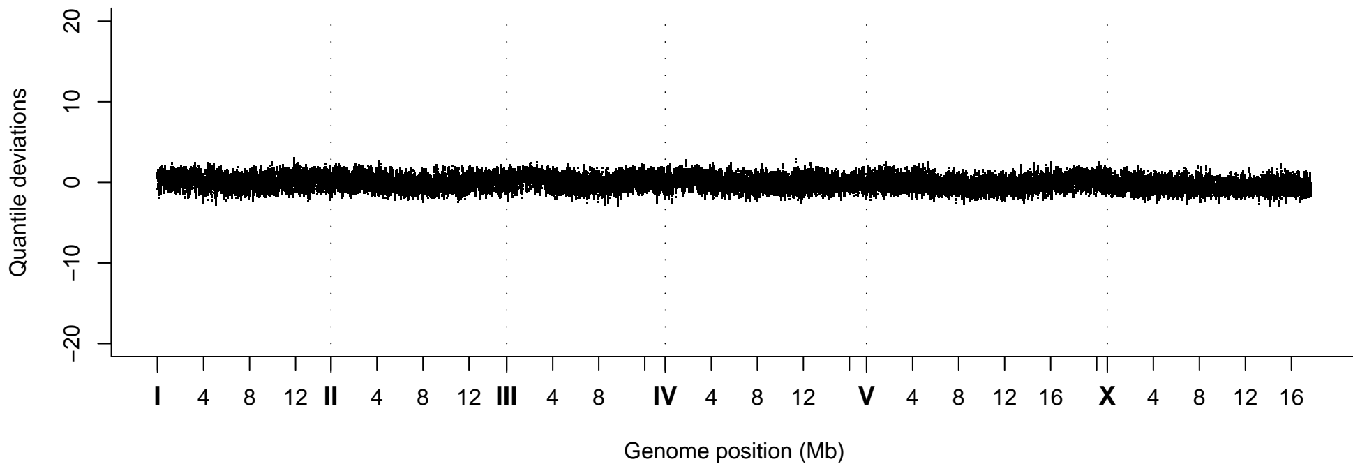
Quantile Deviations, Strain VC20278
