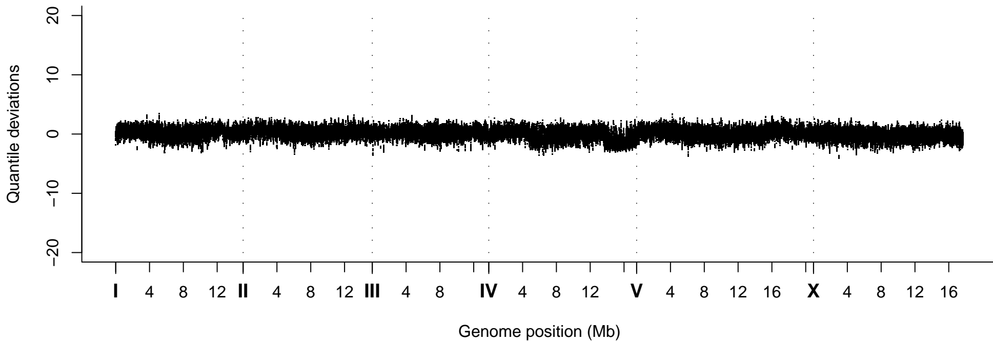
Quantile Deviations, Strain VC20288
