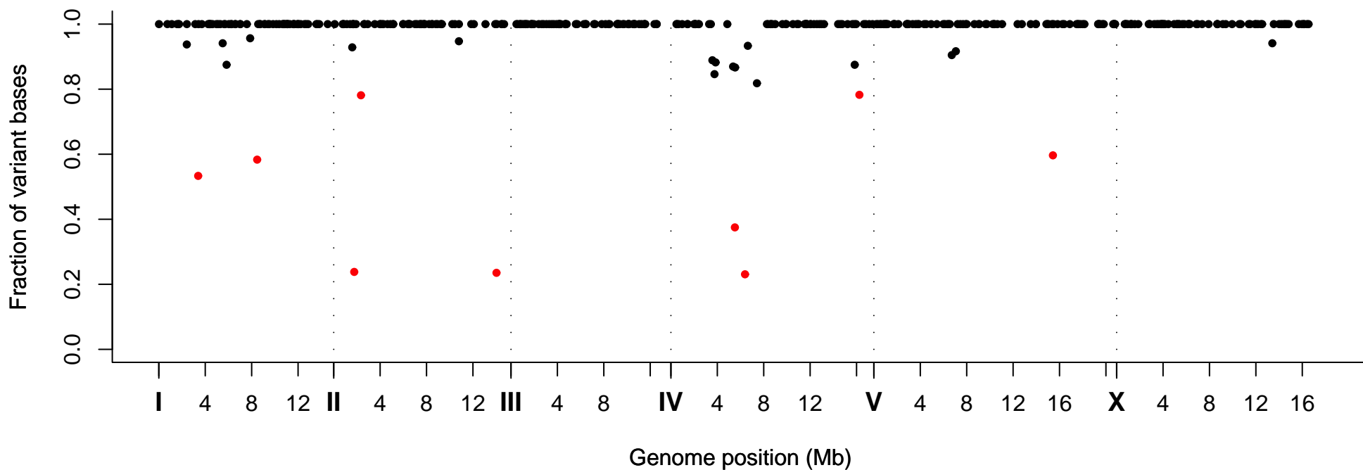
Fraction of Variant Bases at Position, Strain VC20288
