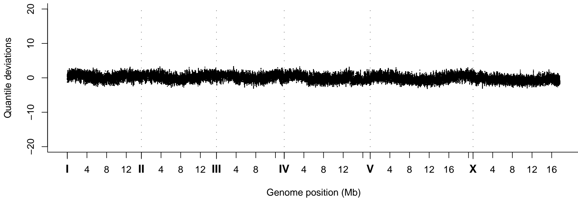
Quantile Deviations, Strain VC20301
