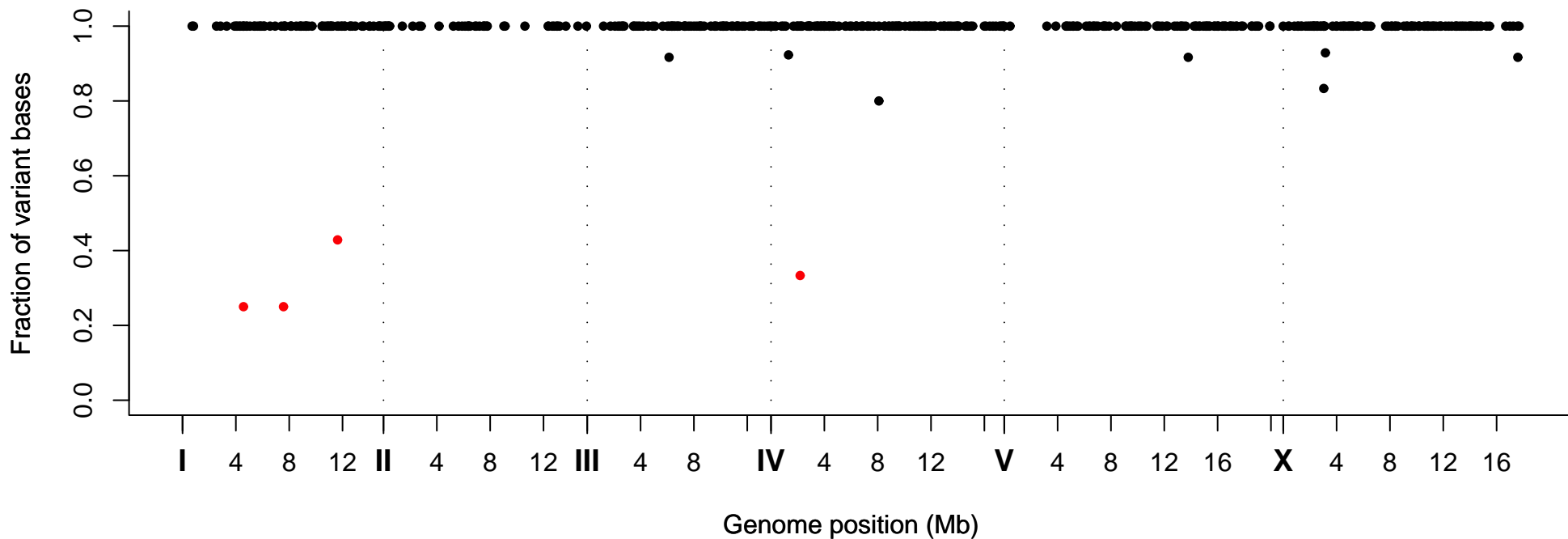
Fraction of Variant Bases at Position, Strain VC20301
