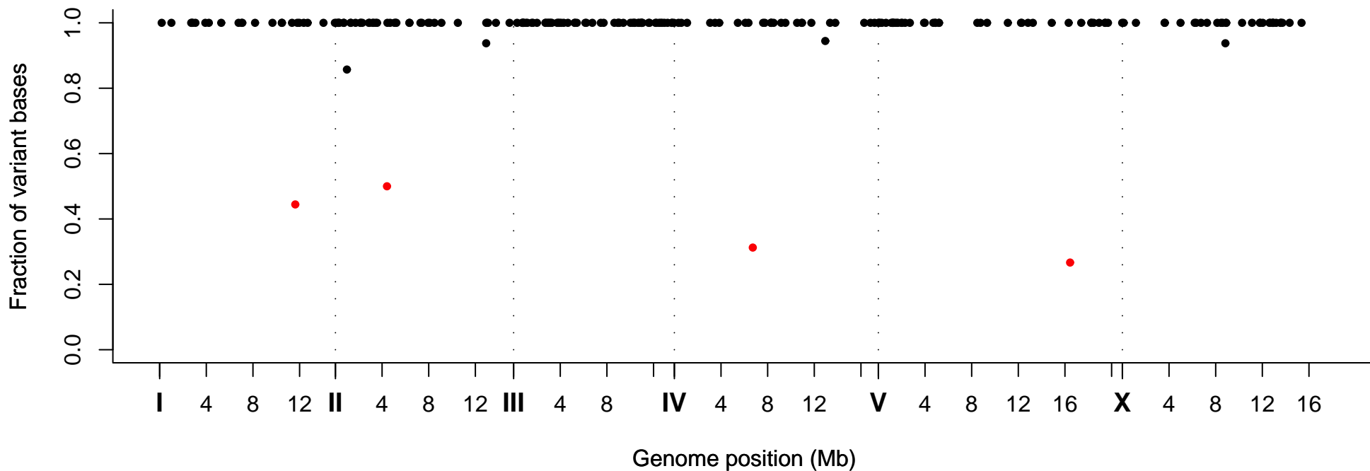
Fraction of Variant Bases at Position, Strain VC20323
