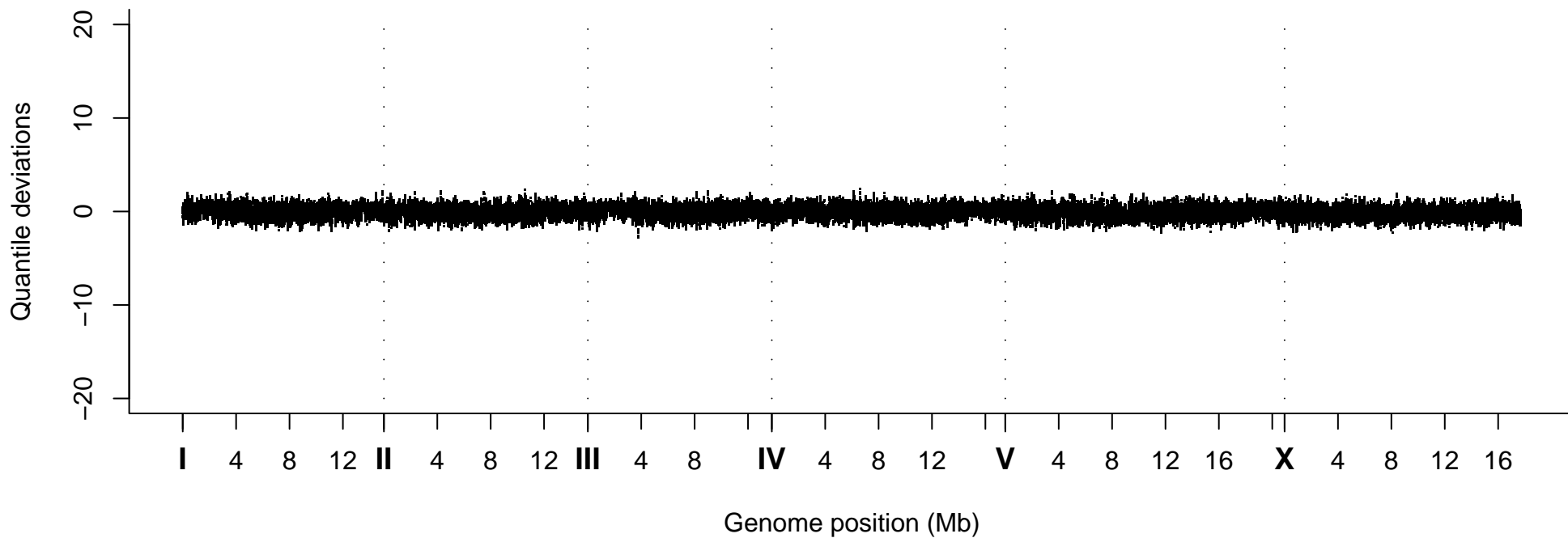
Quantile Deviations, Strain VC20323
