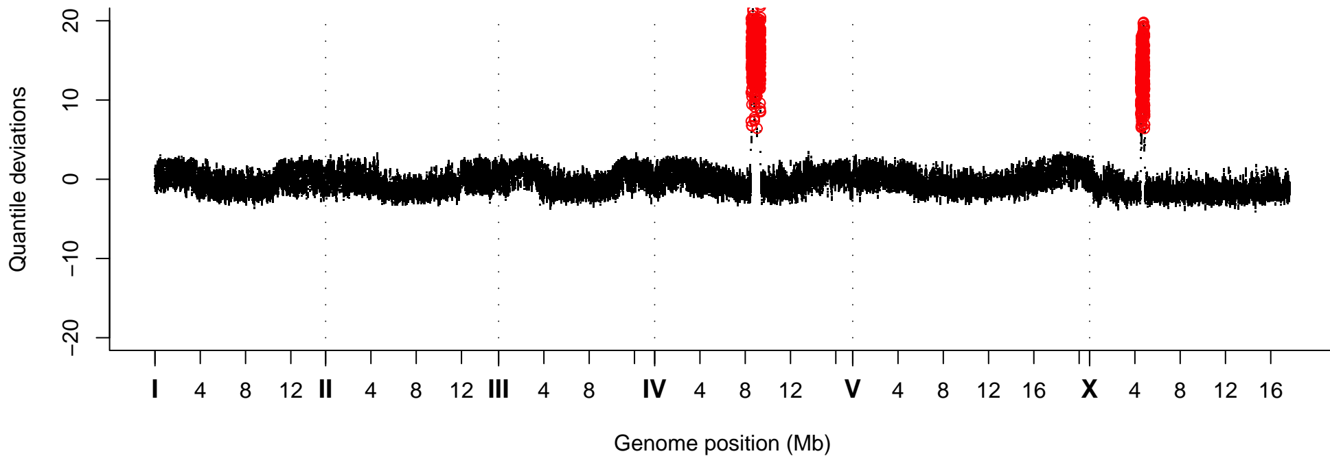
Quantile Deviations, Strain VC20327
