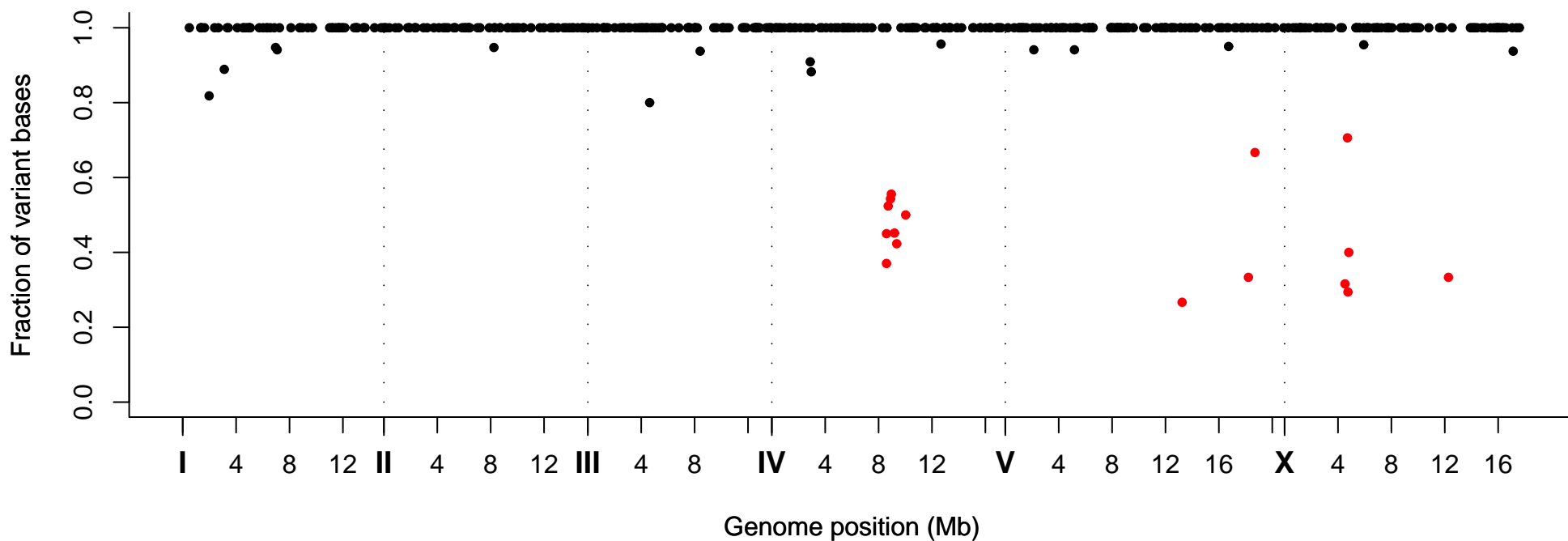
Fraction of Variant Bases at Position, Strain VC20327
