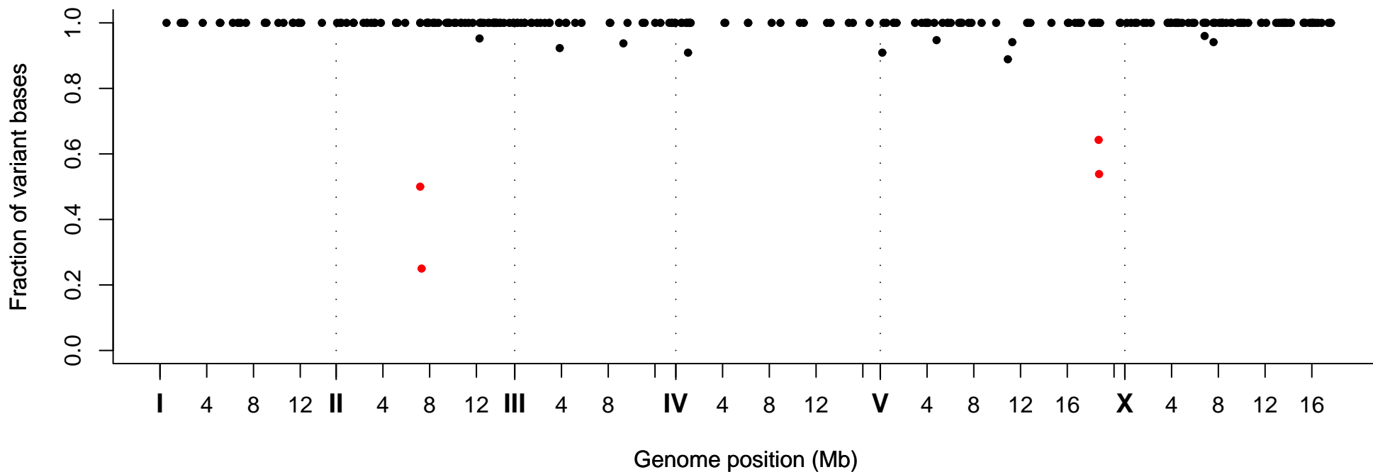
Fraction of Variant Bases at Position, Strain VC20328
