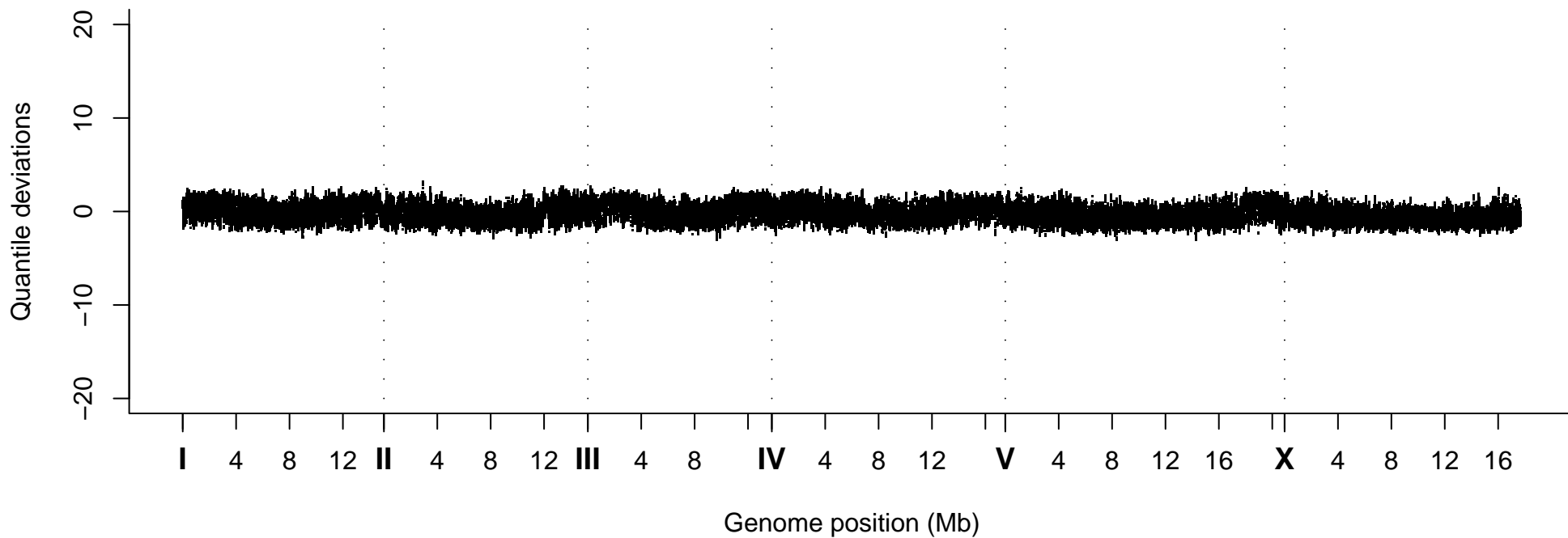
Quantile Deviations, Strain VC20328
