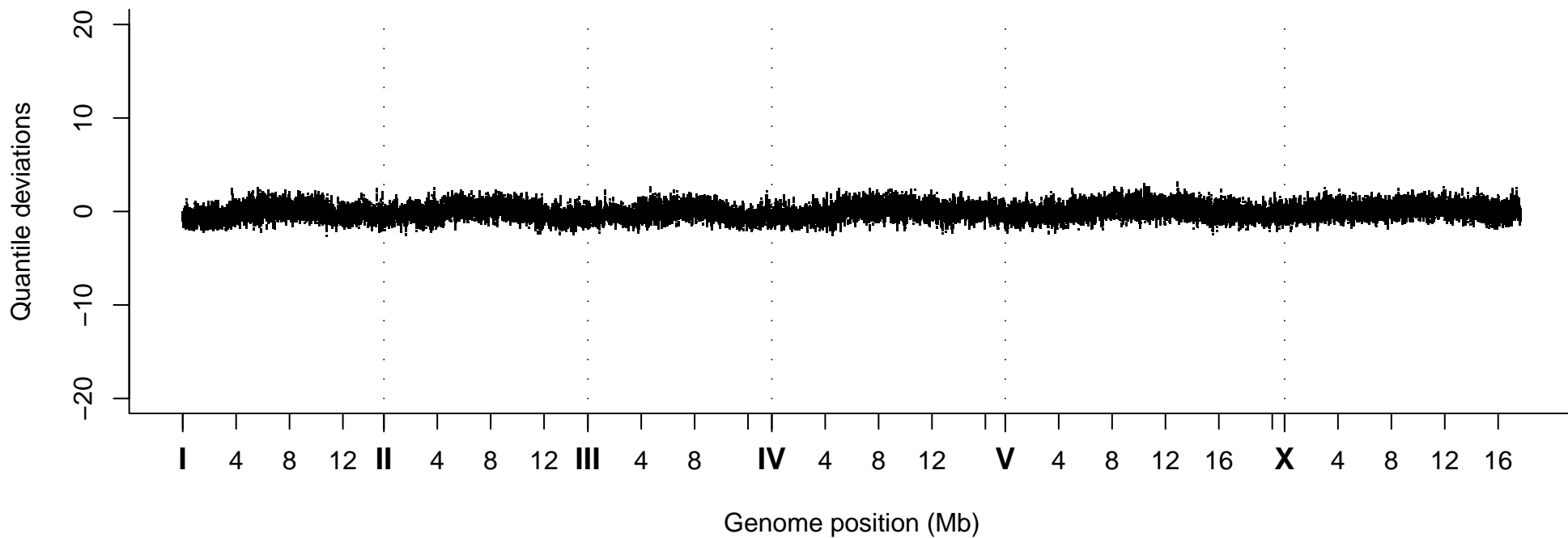
Quantile Deviations, Strain VC20331
