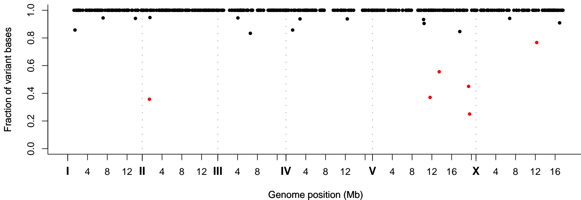
Fraction of Variant Bases at Position, Strain VC20331
