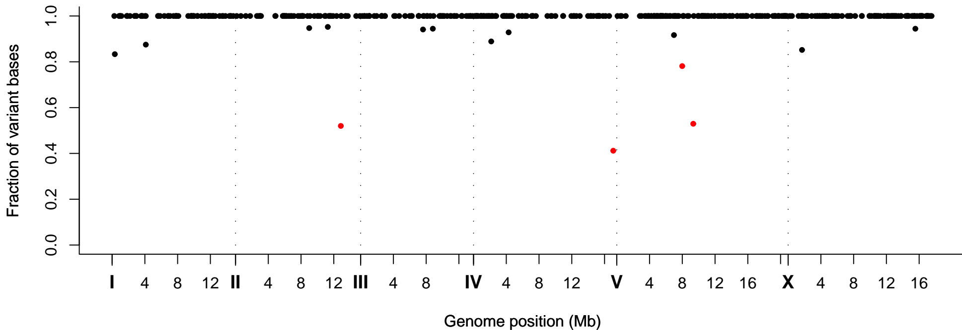
Fraction of Variant Bases at Position, Strain VC20333
