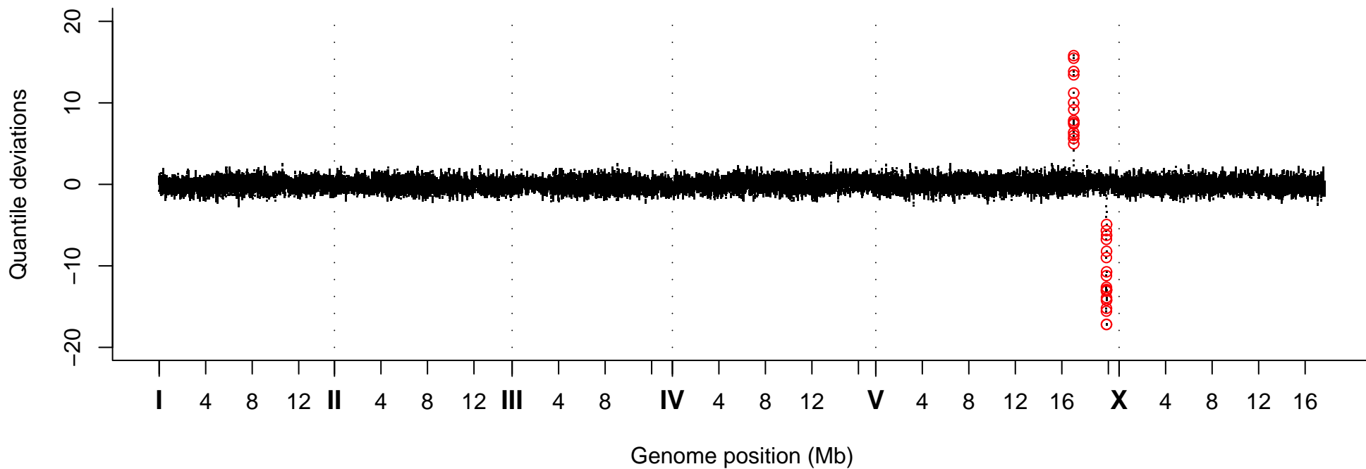
Quantile Deviations, Strain VC20333
