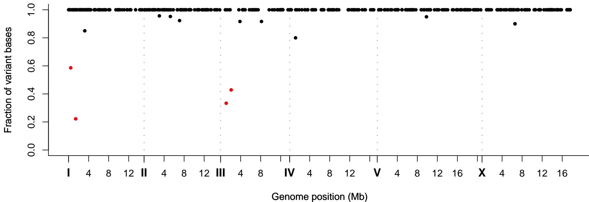
Fraction of Variant Bases at Position, Strain VC20338
