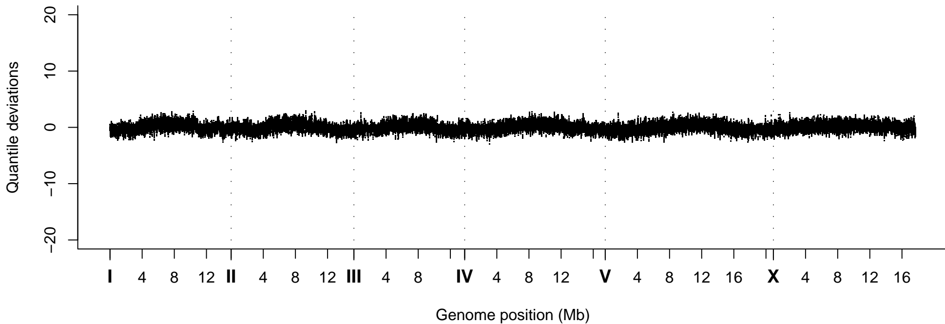
Quantile Deviations, Strain VC20338
