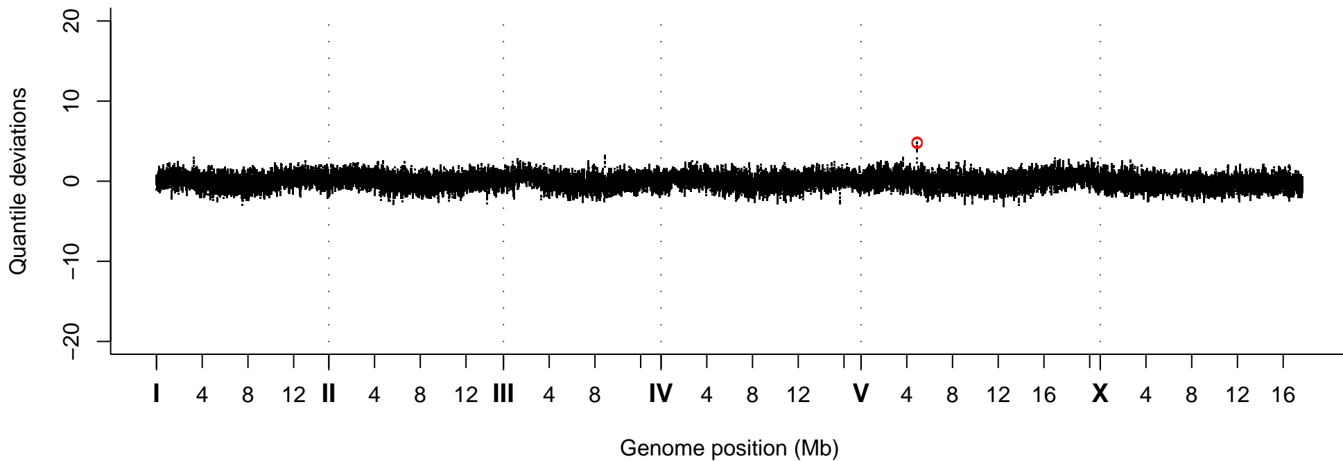
Quantile Deviations, Strain VC20342
