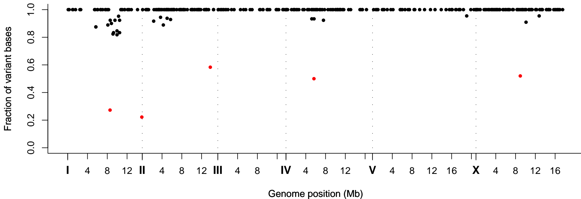
Fraction of Variant Bases at Position, Strain VC20342
