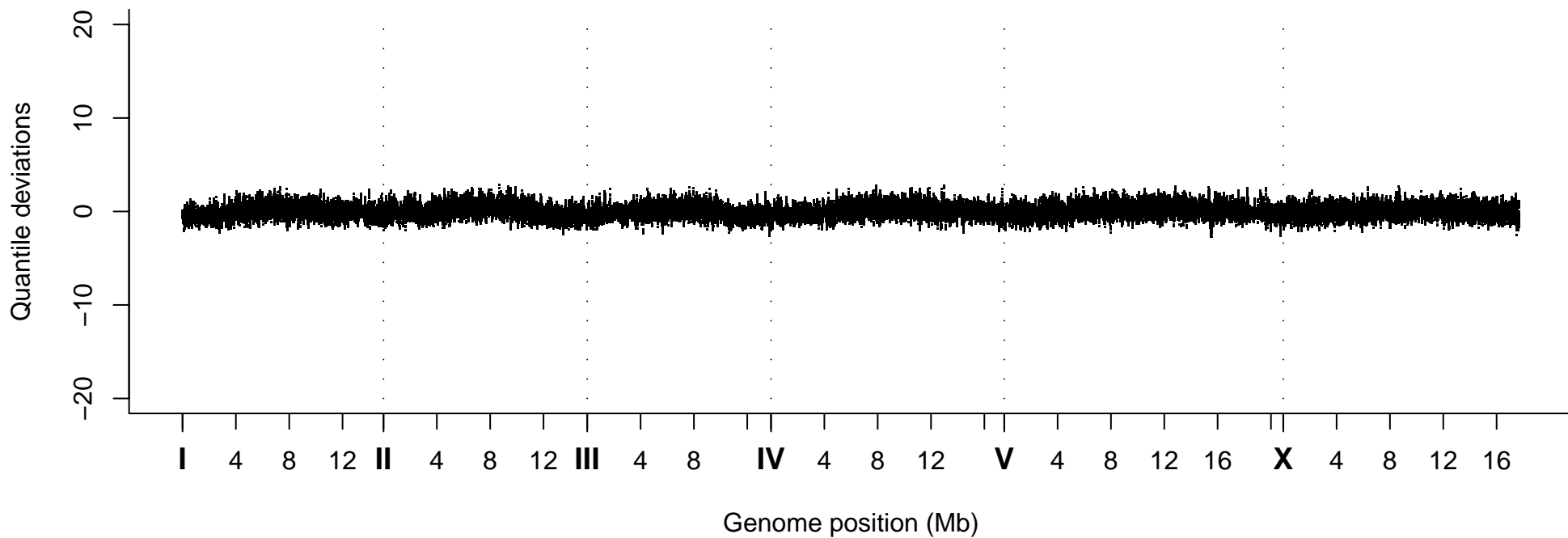
Quantile Deviations, Strain VC20345
