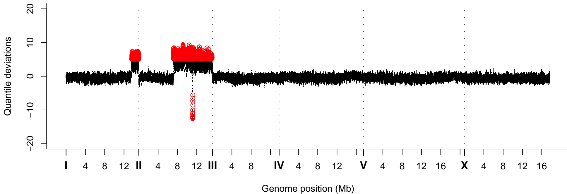
Quantile Deviations, Strain VC20350
