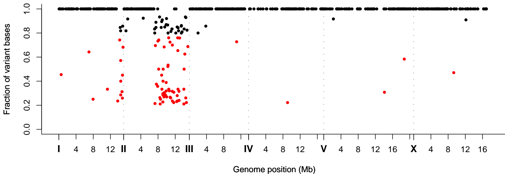
Fraction of Variant Bases at Position, Strain VC20350
