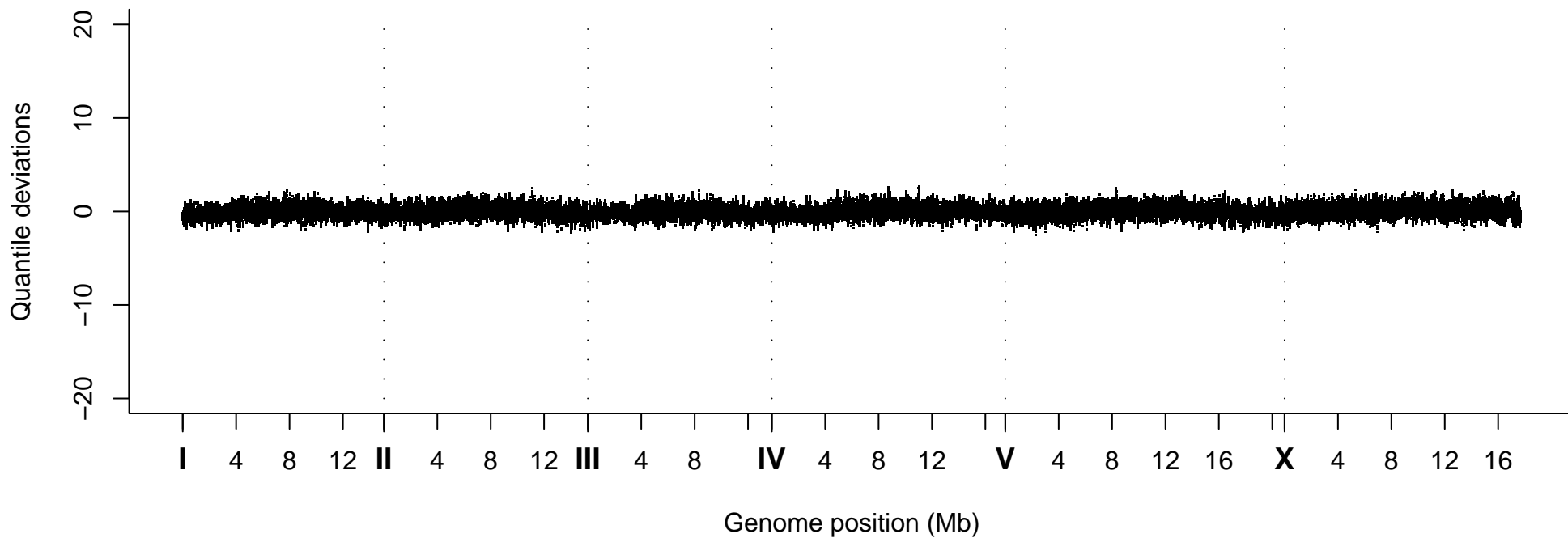
Quantile Deviations, Strain VC20355
