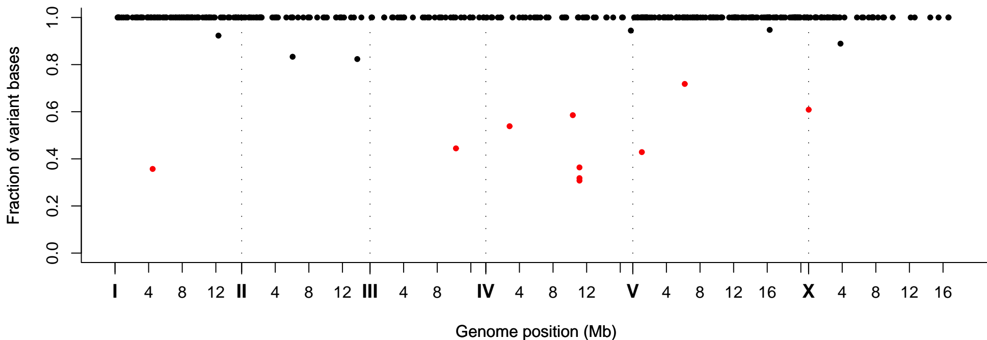
Fraction of Variant Bases at Position, Strain VC20355
