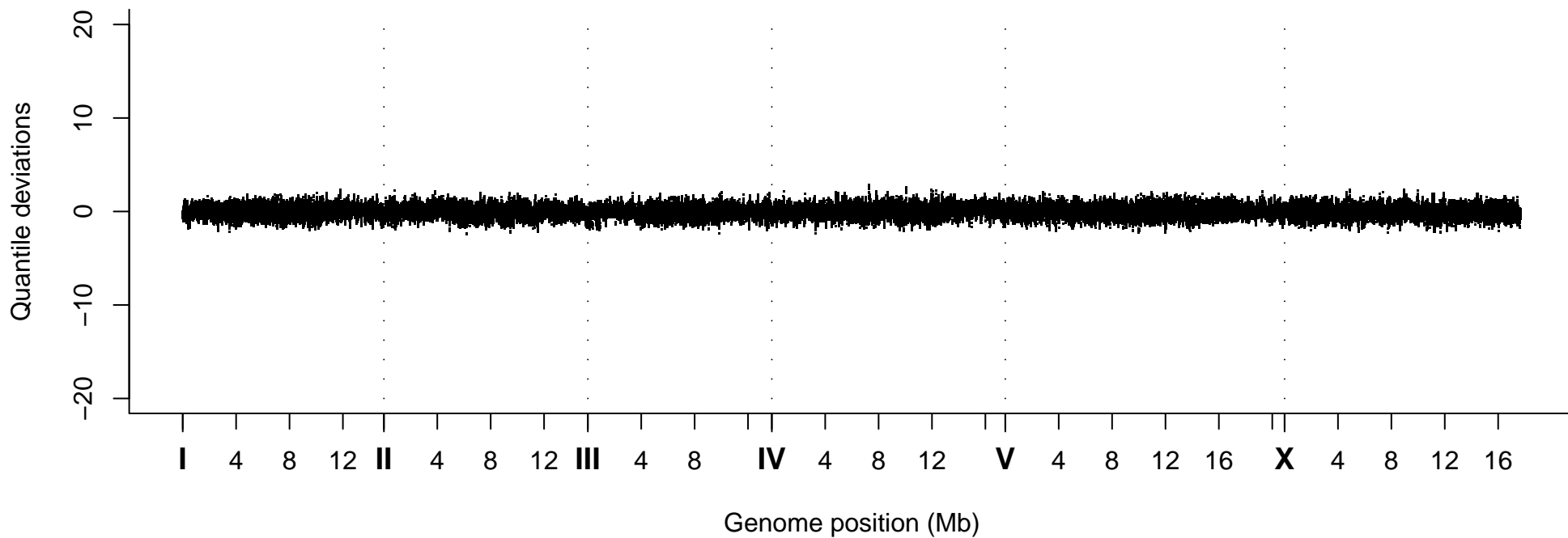
Quantile Deviations, Strain VC20357
