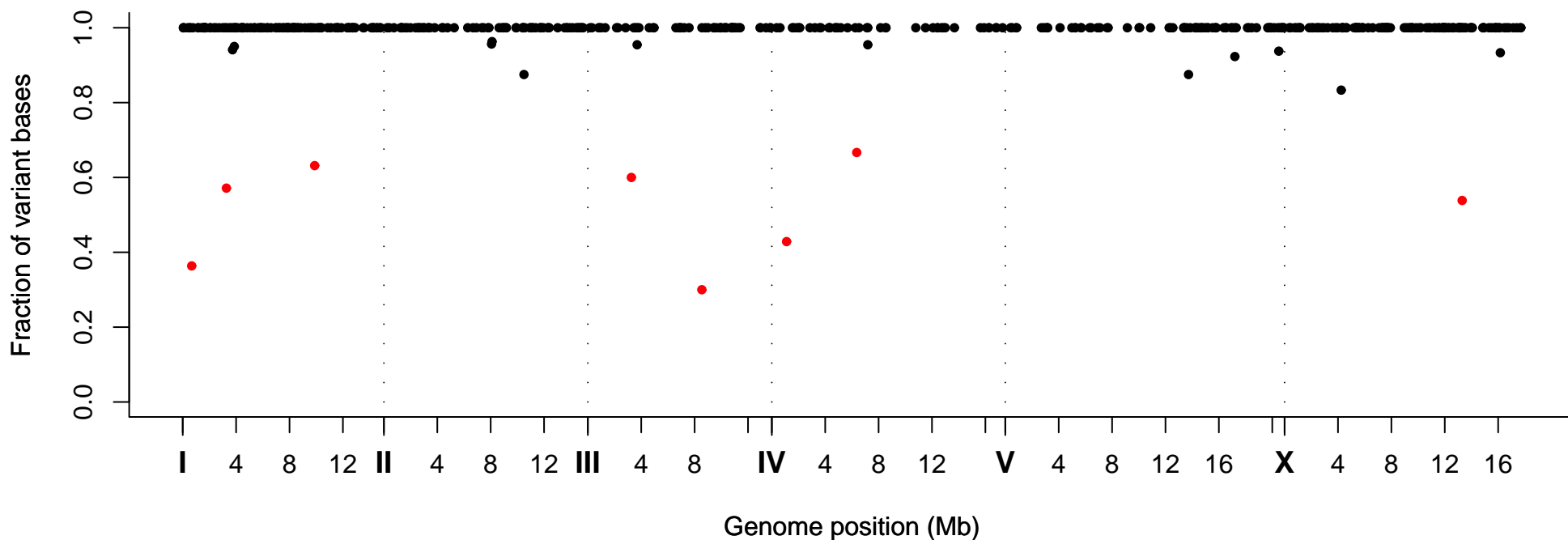
Fraction of Variant Bases at Position, Strain VC20357
