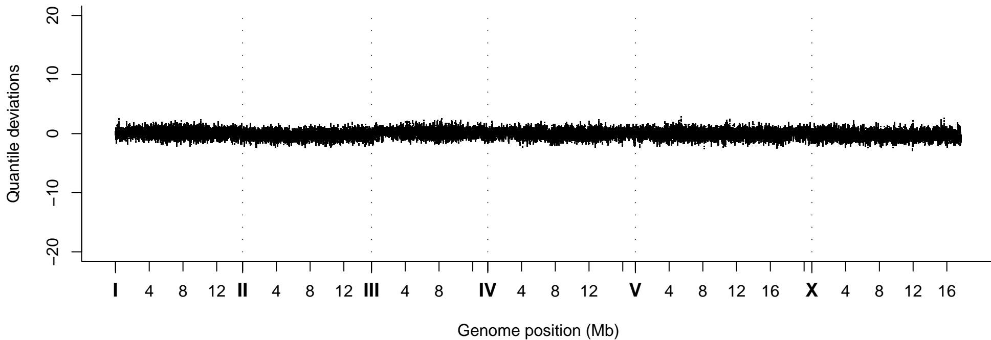
Quantile Deviations, Strain VC20370
