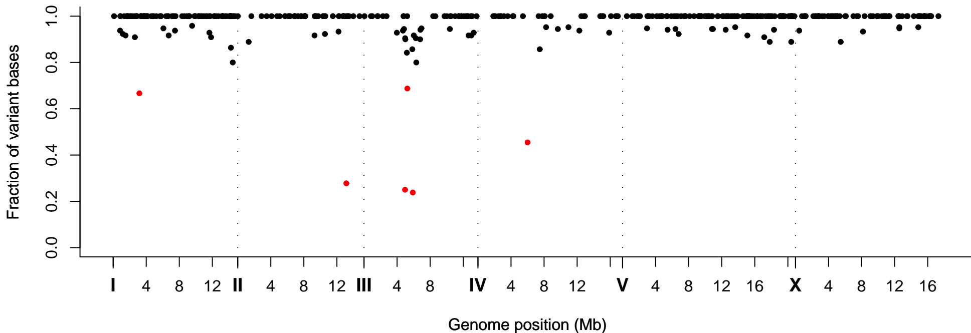
Fraction of Variant Bases at Position, Strain VC20370
