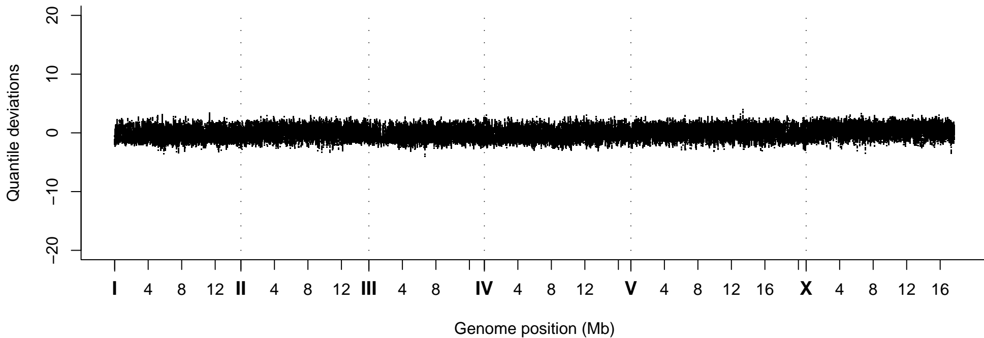
Quantile Deviations, Strain VC20371
