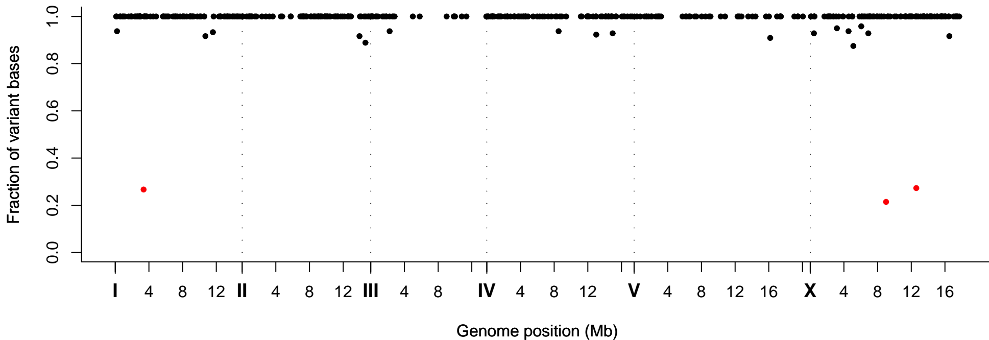
Fraction of Variant Bases at Position, Strain VC20371
