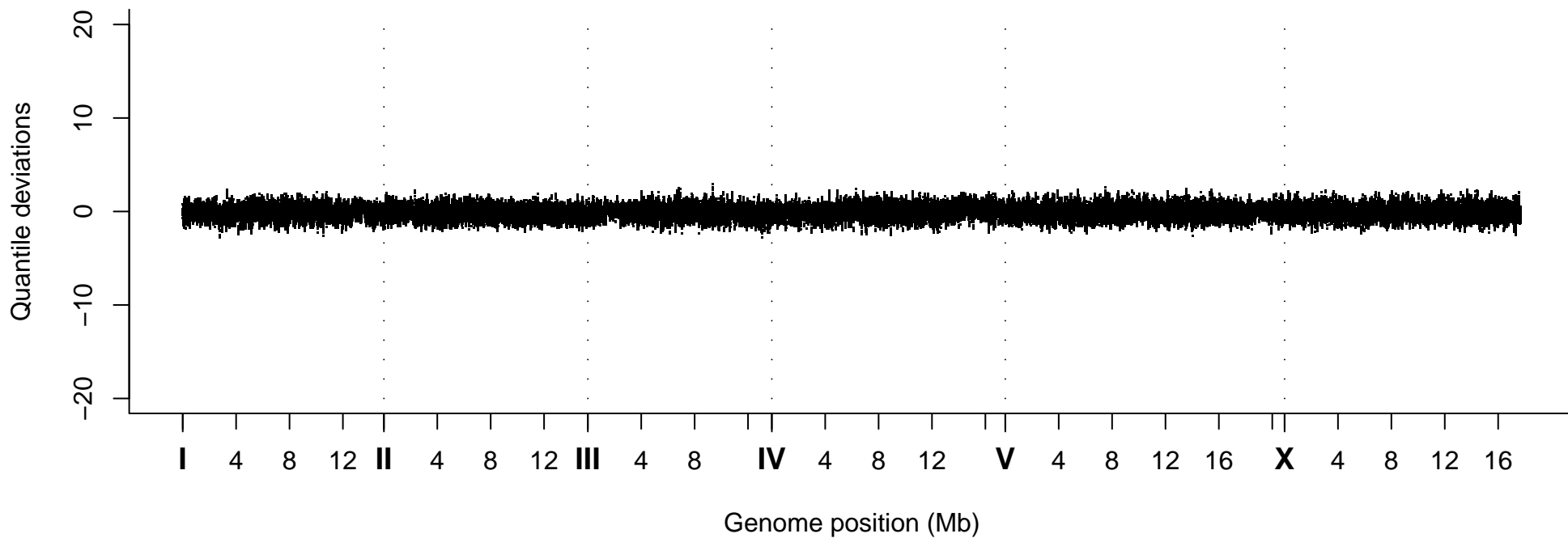
Quantile Deviations, Strain VC20372
