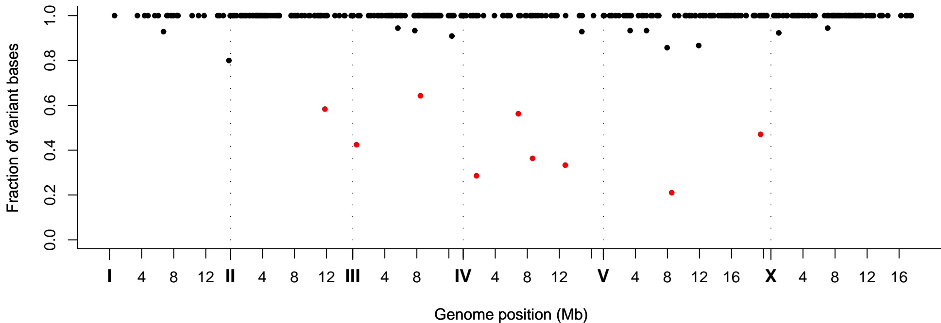
Fraction of Variant Bases at Position, Strain VC20372
