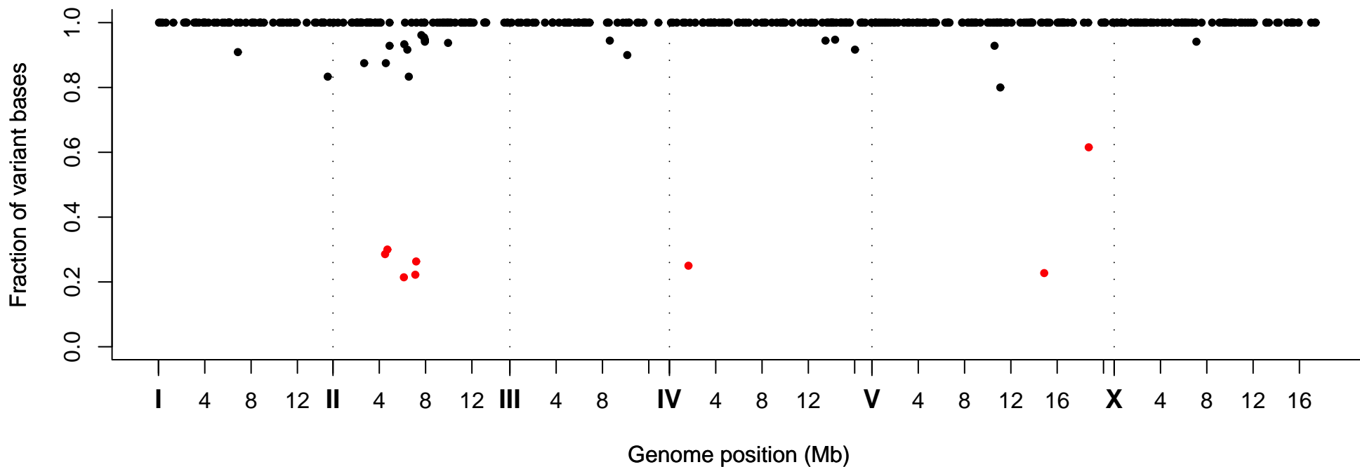
Fraction of Variant Bases at Position, Strain VC20374
