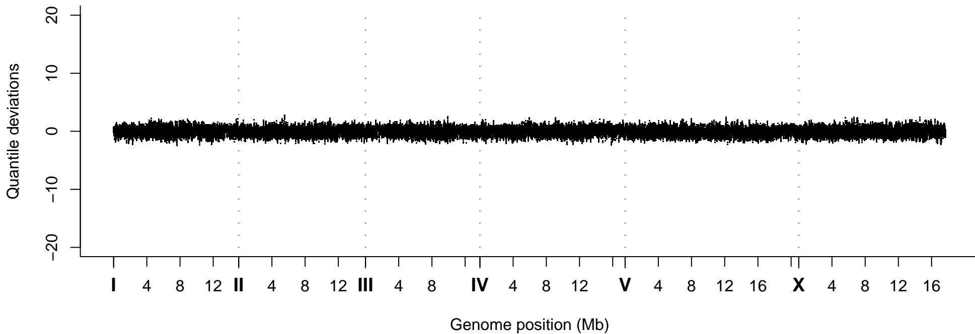
Quantile Deviations, Strain VC20374
