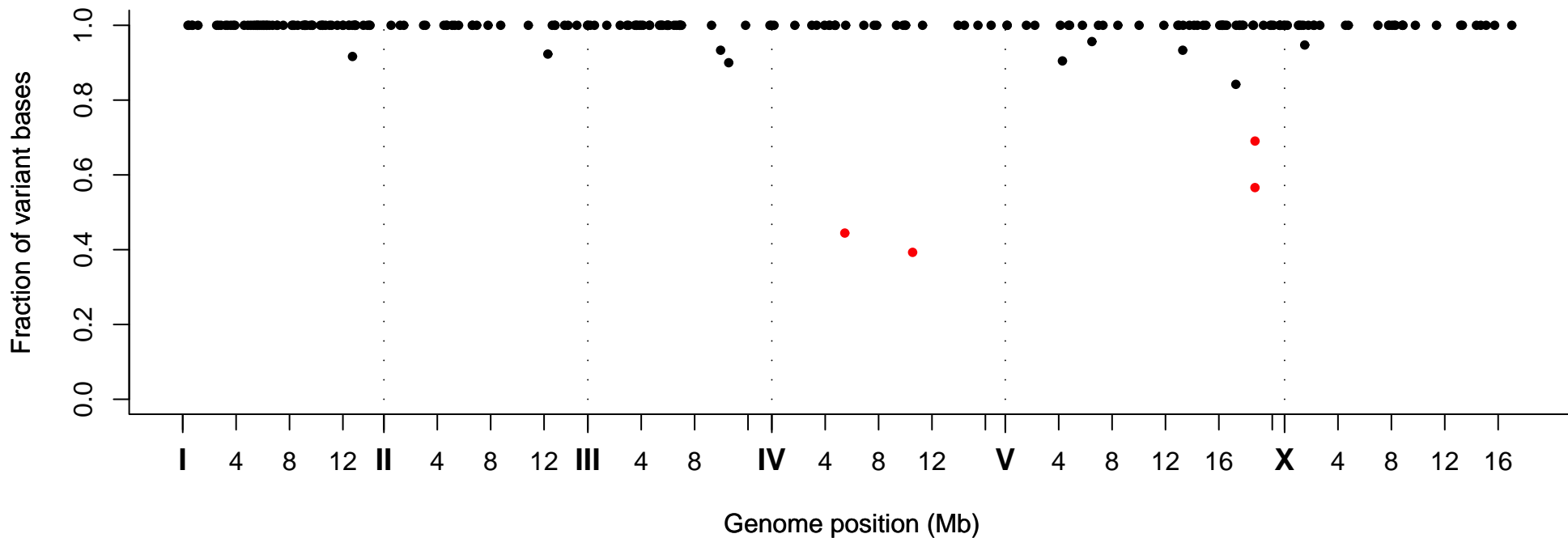
Fraction of Variant Bases at Position, Strain VC20381
