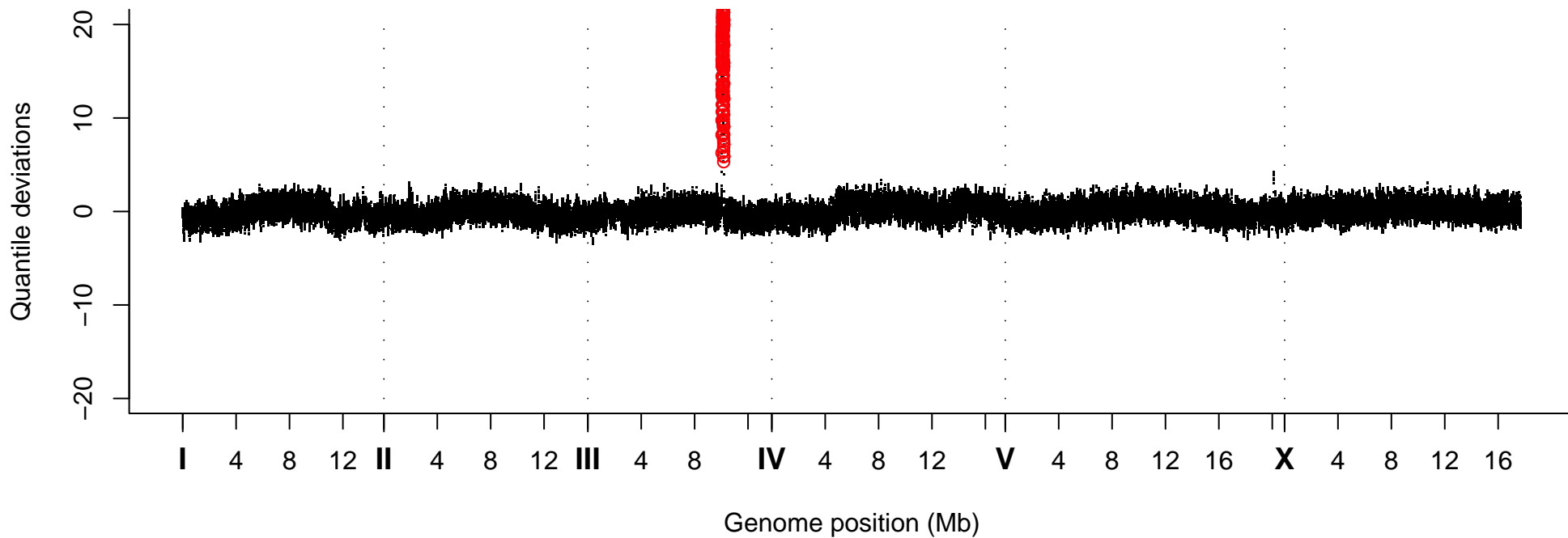
Quantile Deviations, Strain VC20381
