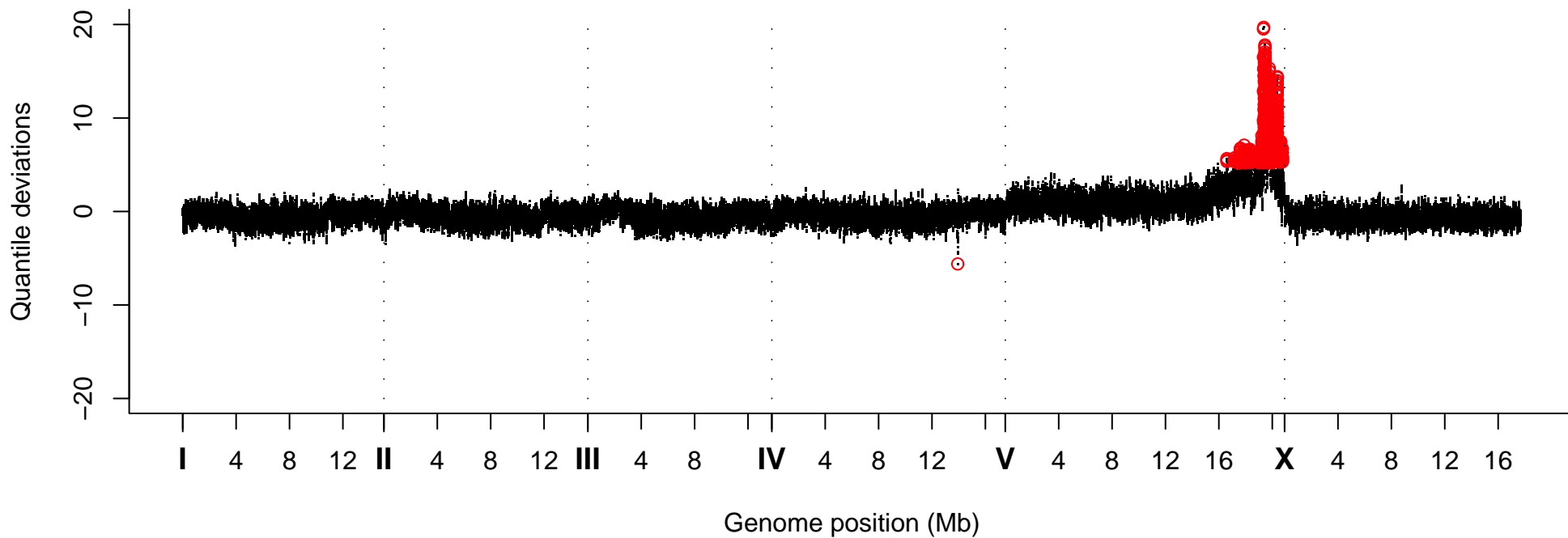
Quantile Deviations, Strain VC20382
