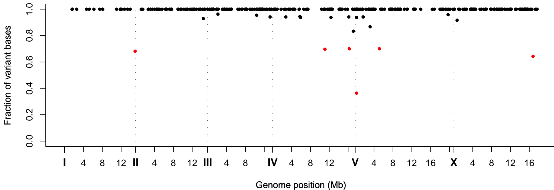
Fraction of Variant Bases at Position, Strain VC20382
