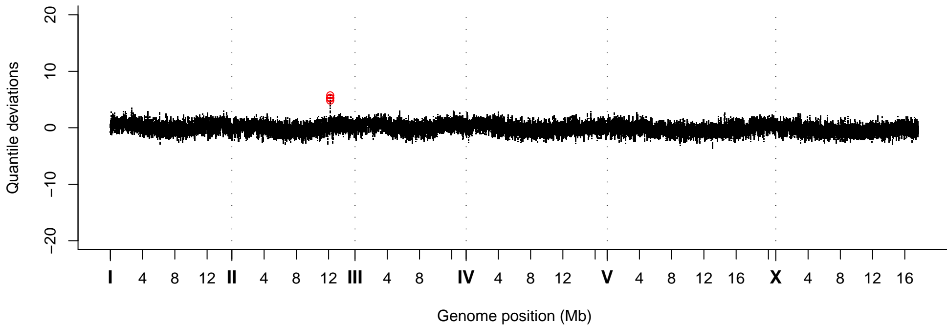
Quantile Deviations, Strain VC20391
