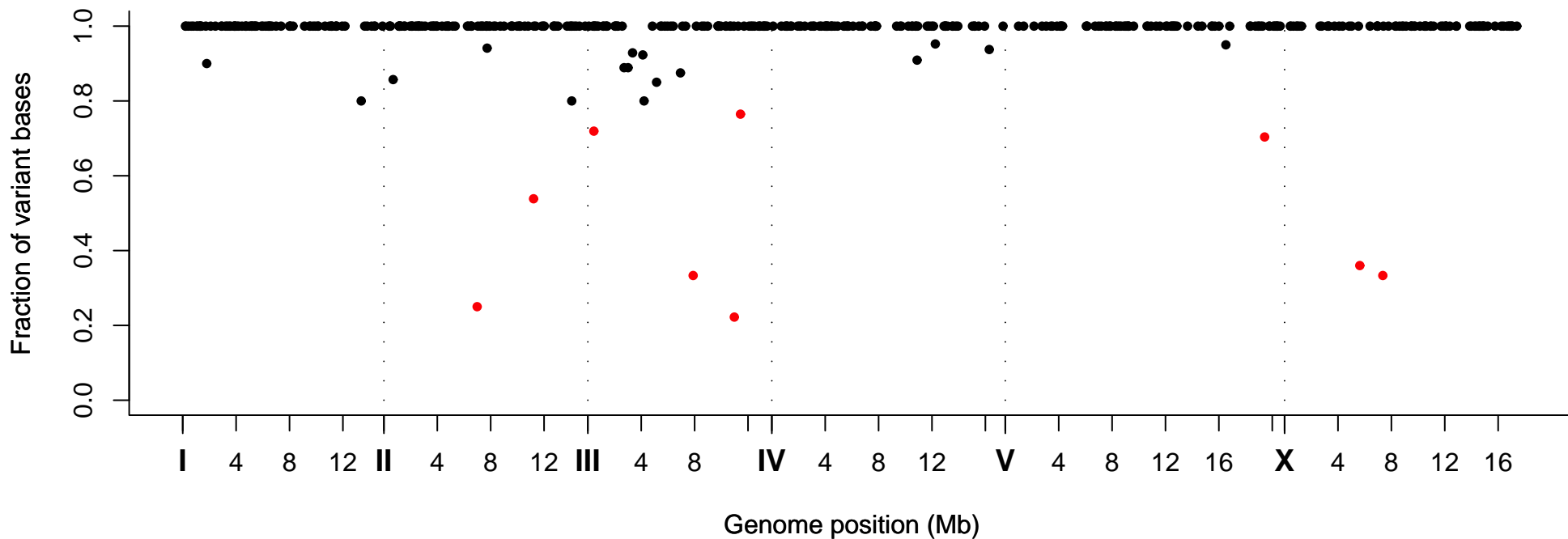
Fraction of Variant Bases at Position, Strain VC20391
