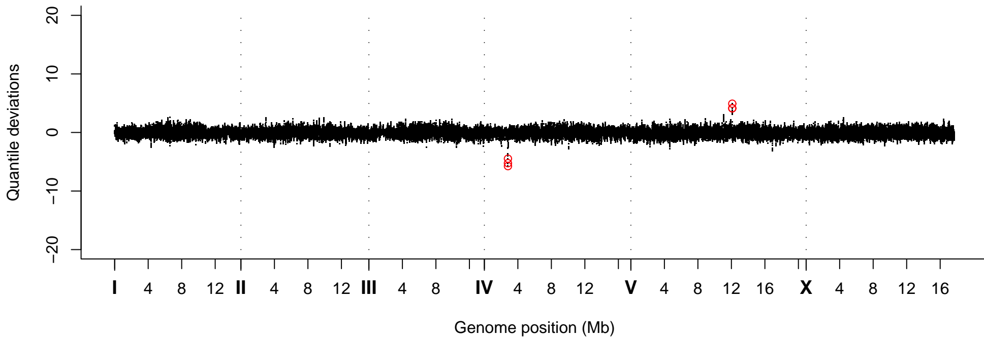
Quantile Deviations, Strain VC20394
