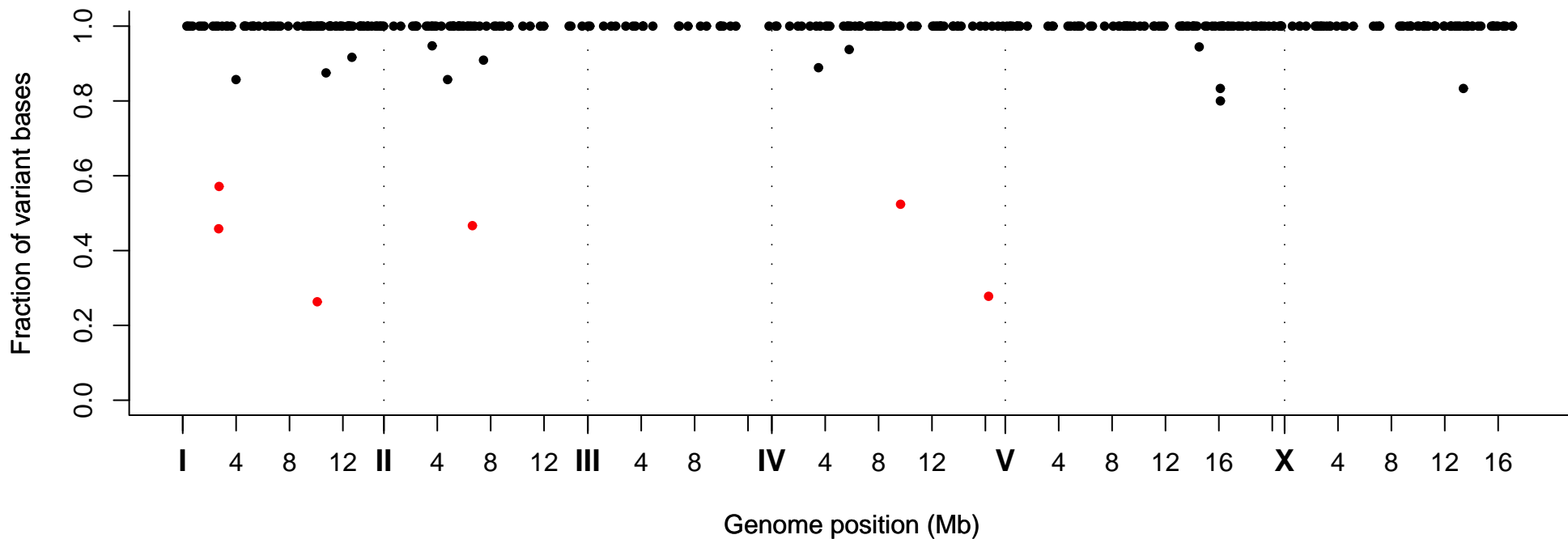
Fraction of Variant Bases at Position, Strain VC20394
