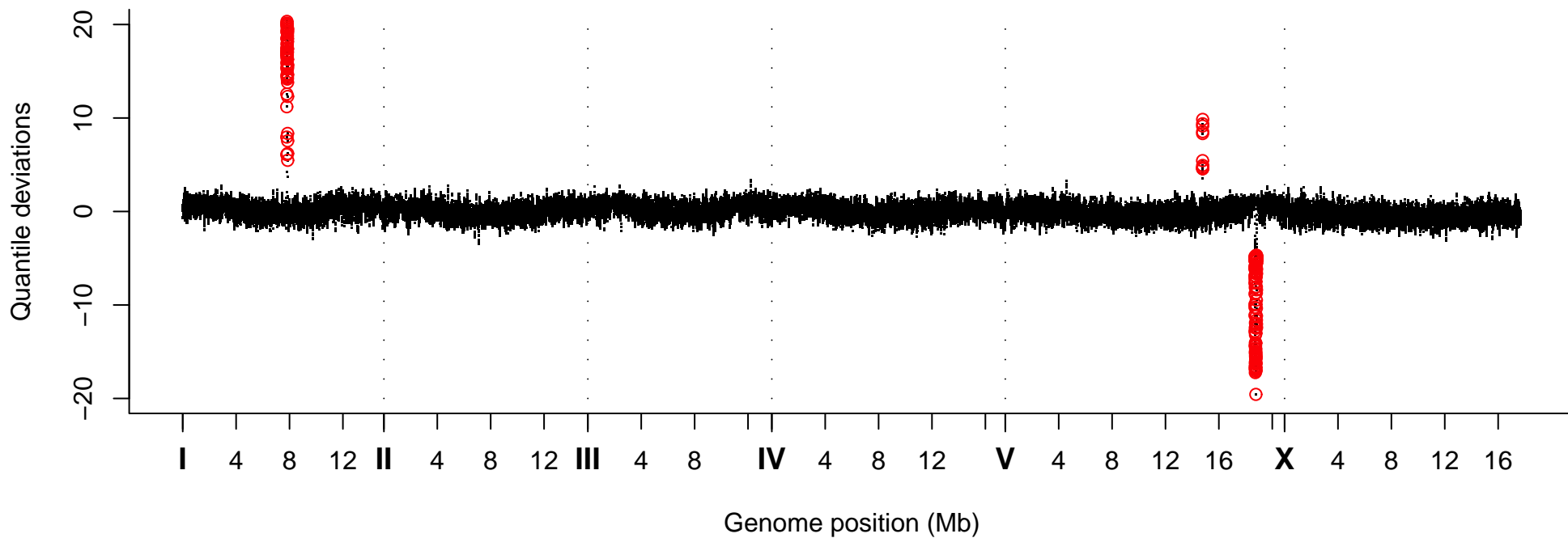
Quantile Deviations, Strain VC20396
