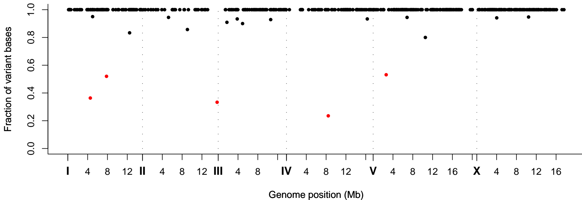
Fraction of Variant Bases at Position, Strain VC20396
