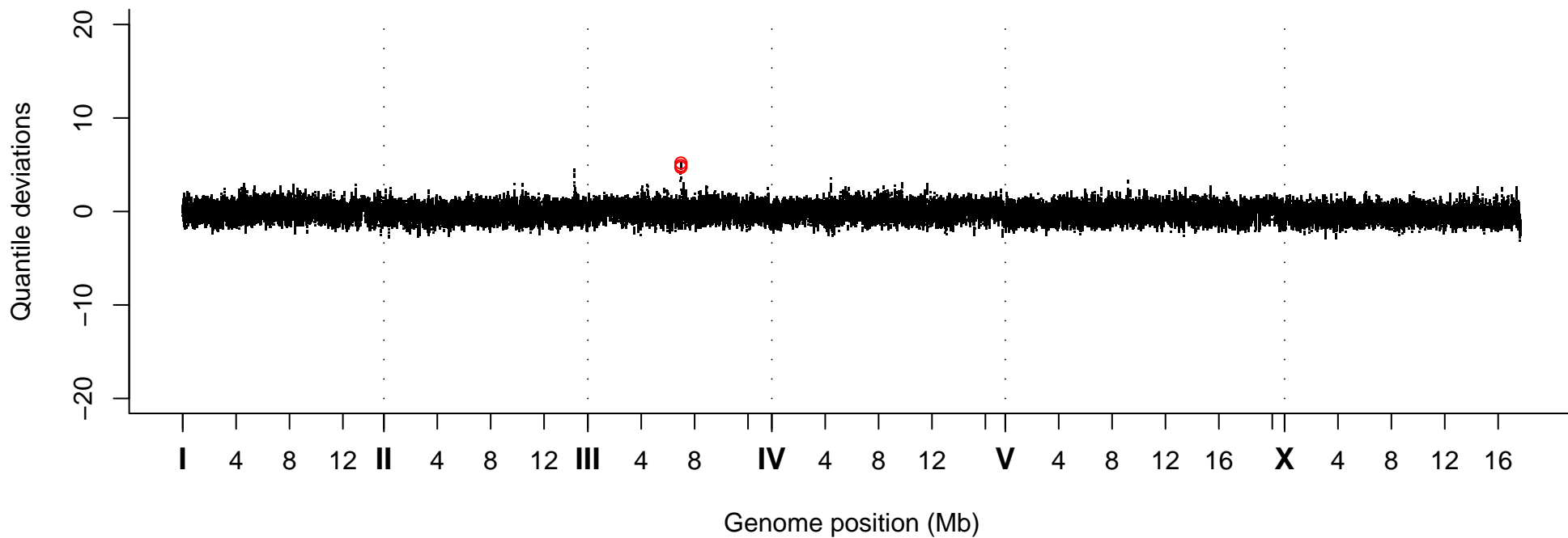
Quantile Deviations, Strain VC20400
