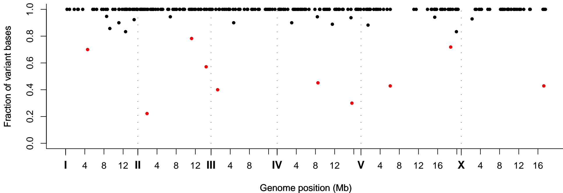
Fraction of Variant Bases at Position, Strain VC20400
