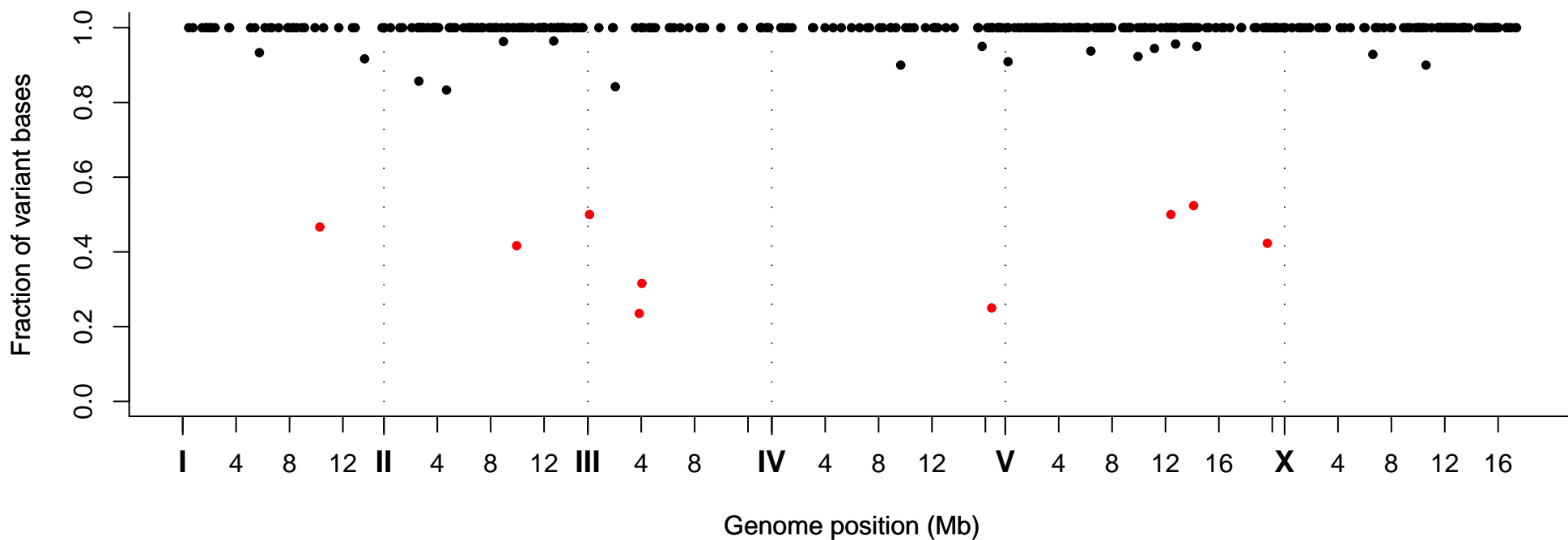
Fraction of Variant Bases at Position, Strain VC20407
