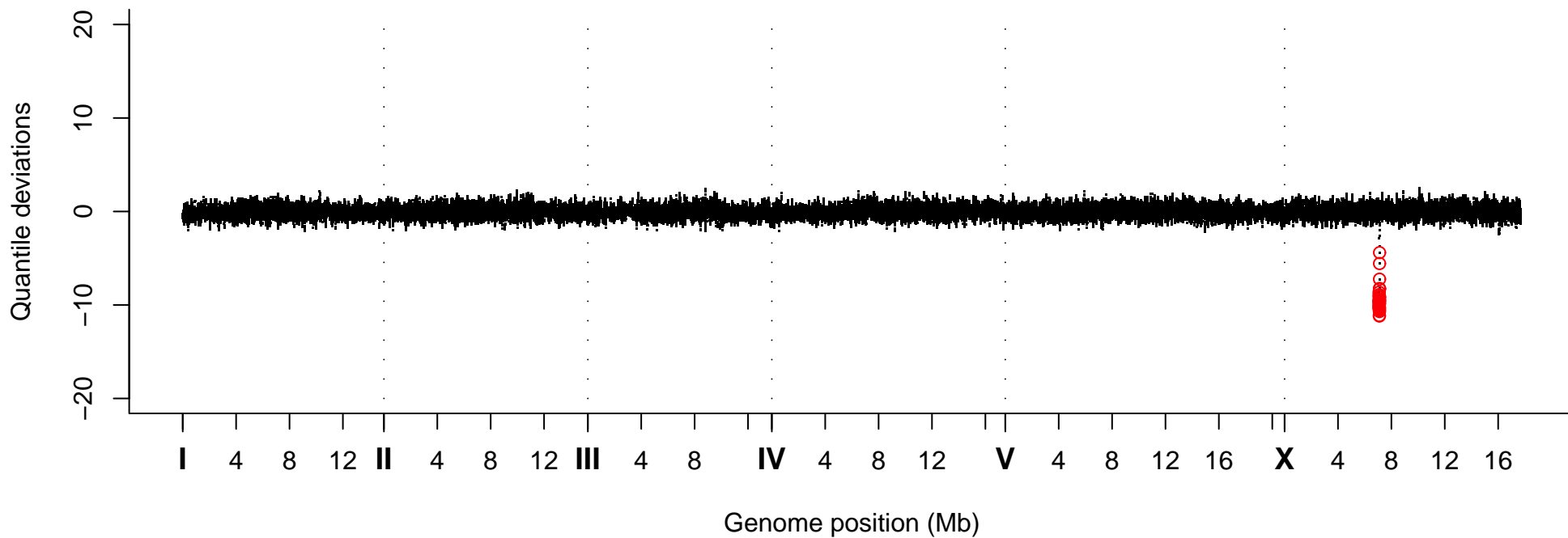
Quantile Deviations, Strain VC20407
