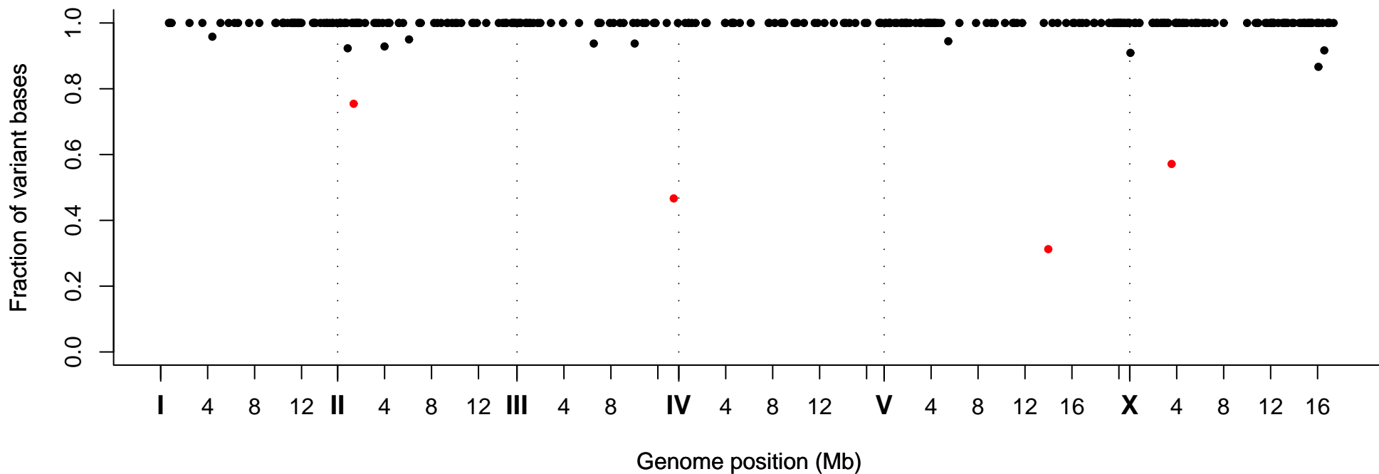
Fraction of Variant Bases at Position, Strain VC20408
