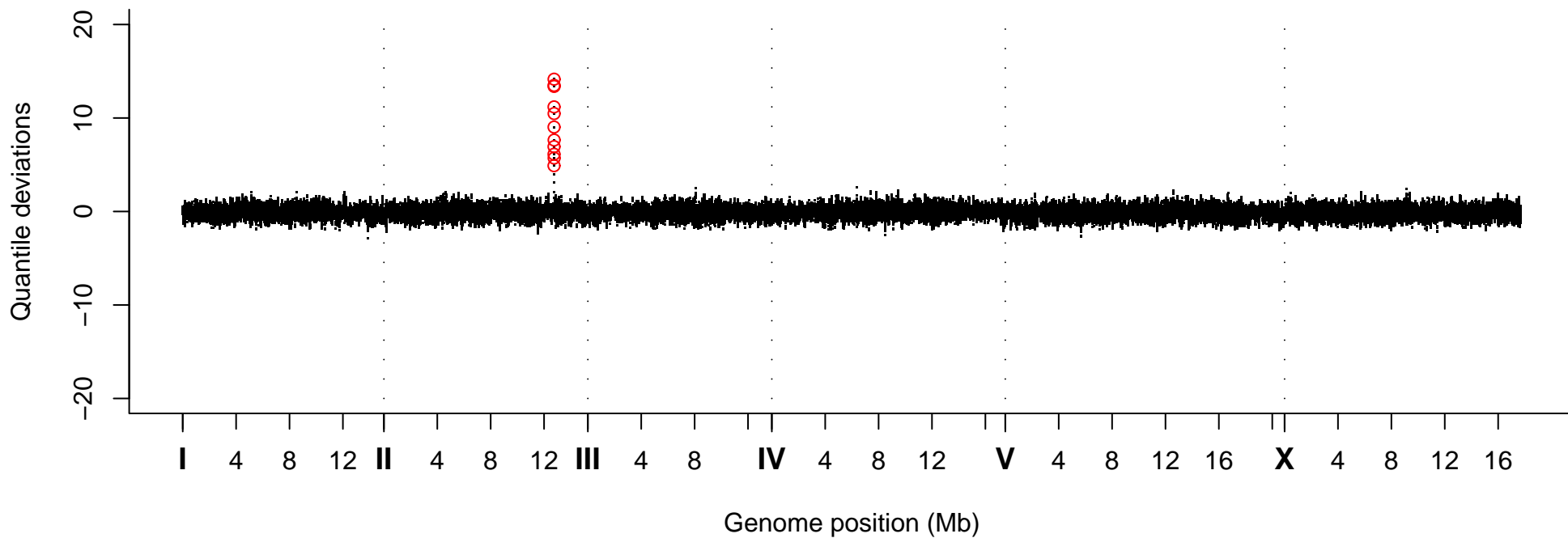
Quantile Deviations, Strain VC20408
