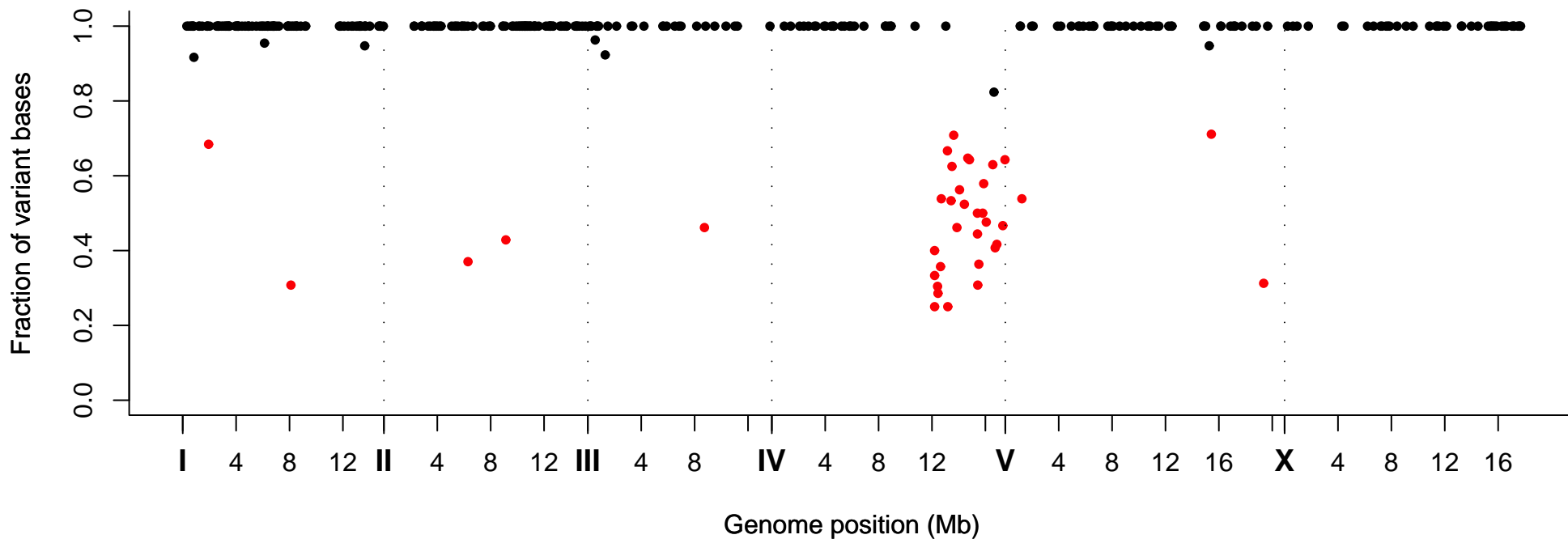
Fraction of Variant Bases at Position, Strain VC20415
